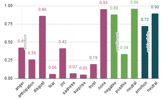
Figure 2: Average AUPRC score of all seven systems in emotion (in purple), sentiment (light green), subjectivity (dark blue) classification.
