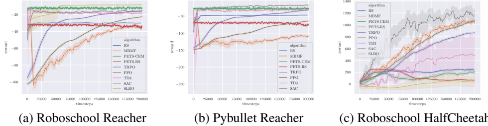
Figure 12: The performance curve for some of the tasks based on Roboschool or Pybullet Klimov &amp; Schulman (2017); AMD (2014); Ellenberger (2018).
