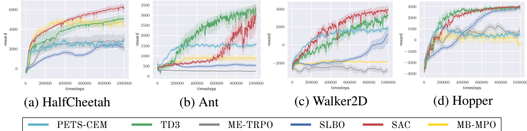
Figure 2: Performance curve for each algorithm trained for 1 million time-steps.
