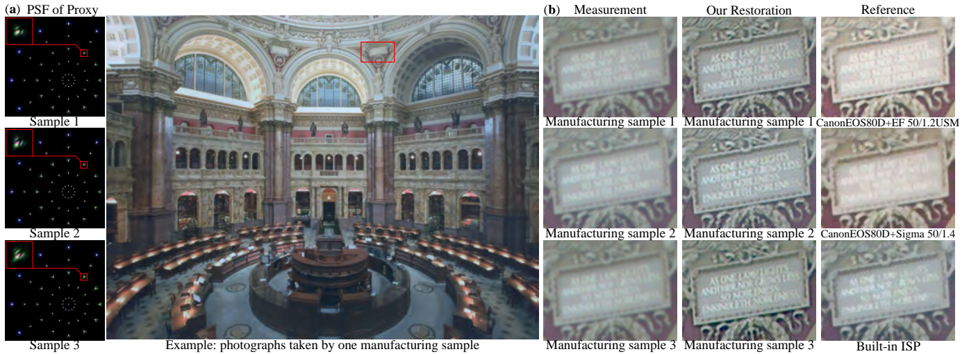
Fig. 1. Manufacturing biases adaptation and comparisons. (a) centrosymmetric PSF calculated by the proxy camera of different machining samples ( Best viewed with zoom ). (b) magnified comparisons of the photographs taken in the same scene. We show the measured degradation of each Phone (converted to sRGB for visualization) and our restoration output from the same ISP pipeline. And the results of high-end DSLR cameras are shown for reference (captured under same aperture for comparisons).
