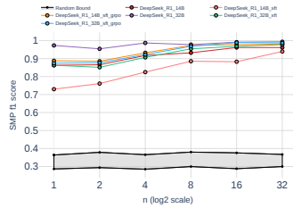
Figure 13: Ground truth hold results on Fin-2024[December]
