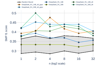
Figure 11: OOD_Stock&Date results on Fin-2024[December]
