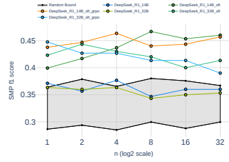
Figure 9: OOD_Stock results on Fin-2024[December]
