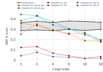
Figure 14: Ground truth down results on Fin-2024[December]
