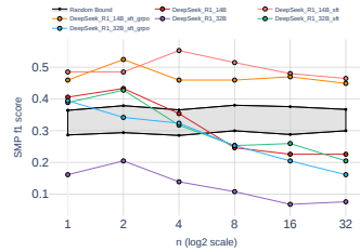
Figure 12: Ground truth up results on Fin-2024[December]
