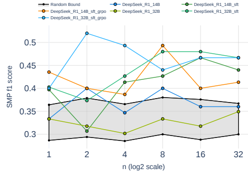
Figure 35: OOD_Stock&Date f1 score results on Fin-20254[June] .
