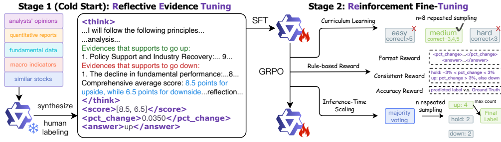
Figure 4: Two-stage stock movement prediction model training framework: Stage 1 (Cold Start) uses multi-source data with human labeling and synthesis pipeline for Reflective Evidence Tuning ; Stage 2 applies Reinforcement Fine-Tuning with curriculum learning, reward shaping, and inference-time scaling for final label determination.
