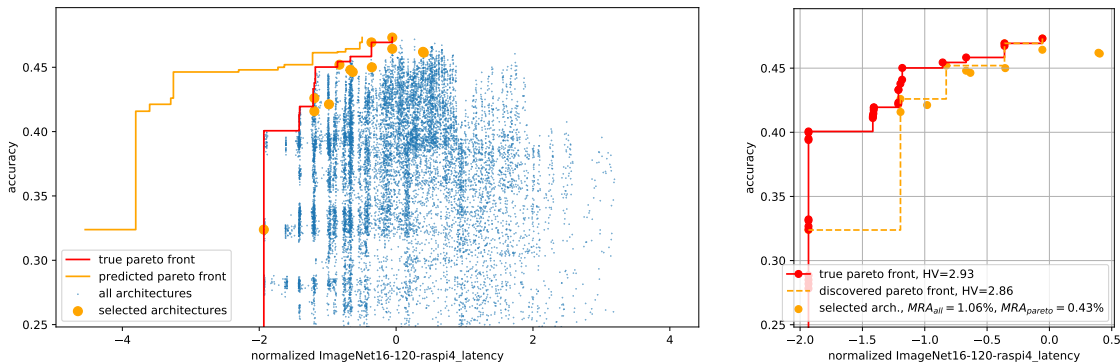
Figure 3: An example of predictor-guided architecture selection, \text{std}=0.5 . Left: The simulated predictor makes an inaccurate latency prediction for each architecture (blue), resulting in the selection of the supposedly-best architectures (orange dots). Even though the predicted Pareto front (orange line) may differ significantly from the ground-truth Pareto front (red line), most selected architectures are close to optimal. Right: Same data as left. Simply accepting all selected architectures results in a Mean Reduction of Accuracy ( MRA ) of 1.06%, while verifying the predictions and discarding inferior results improves that to 0.43%. The hypervolume (HV, area under the Pareto-fronts) is reduced by 0.07.
