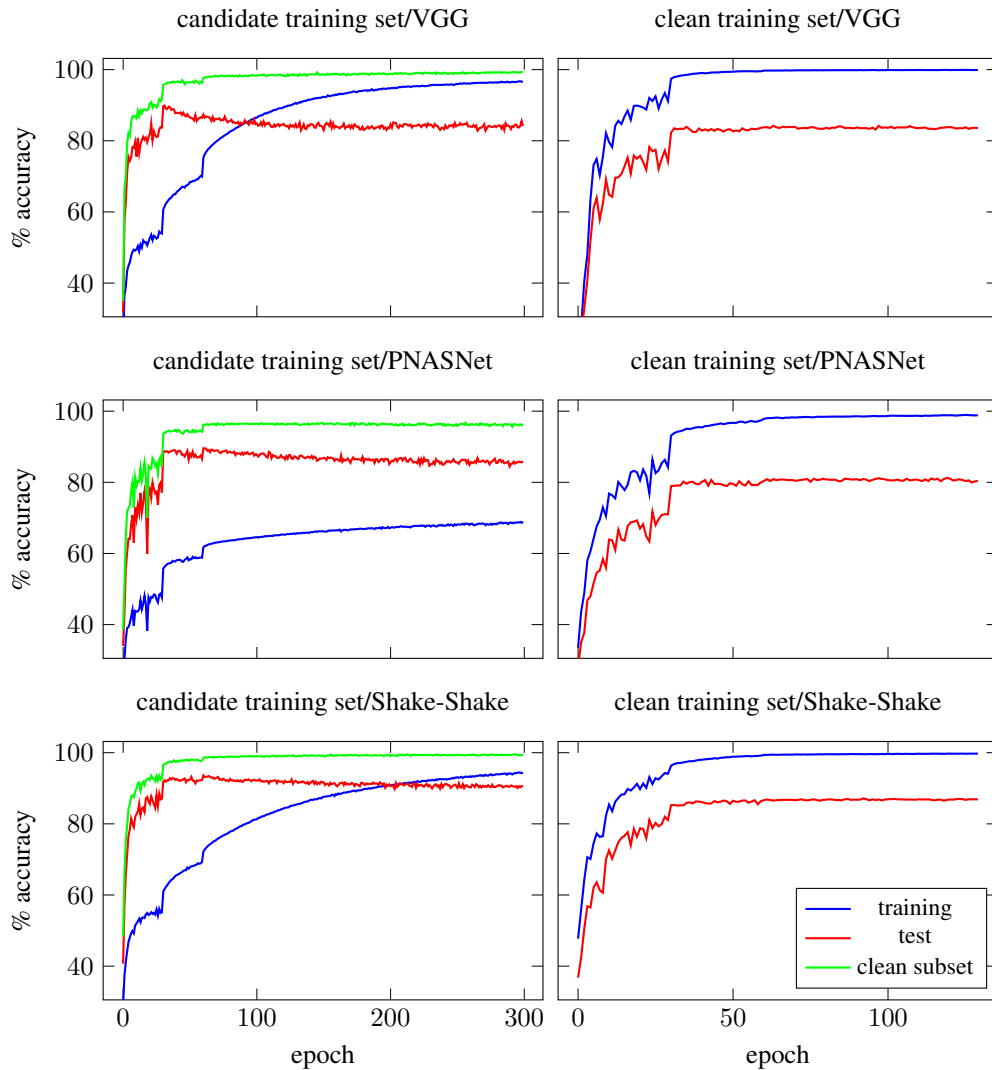
Figure 12: Accuracy on the training set, test set throughout training of the VGG-16, PNASNet, and Shake-Shake-26 2x64d (S-S-I) models on our training set (left) and original CIFAR-10 training set (right). For the experiment on our training set, we also show the accuracy on a subset of the training set that are known to have clean labels and corresponds to CIFAR-10 test set.
