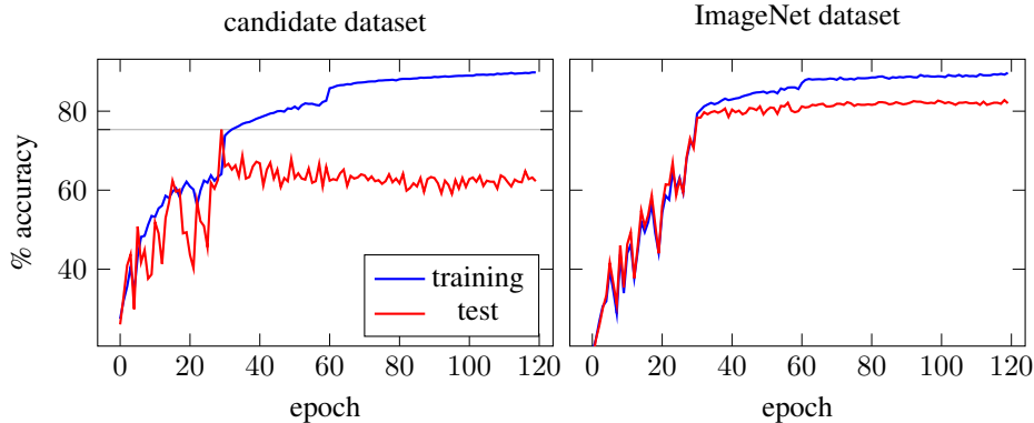
Figure 5: Accuracy on the training set, test set throughout training of the ResNet-18 model on our candidate training set (left) that was obtained from Flickr searches and original ImageNet training set (right) for the classification problem consisting of 15 children classes of the parent class corresponding to invertebrate animals.
