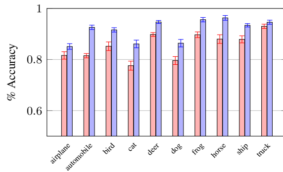
Figure 13: Accuracy per class for training ResNet18 on the original CIFAR-10 training set (red bars) and training on the candidate images with early stopping (blue bars). The plots show that the model trained on the candidate examples has better performance in each class than the model trained on the original training set. The error bars correspond to one standard deviation obtained by averaging over many different initialization.
