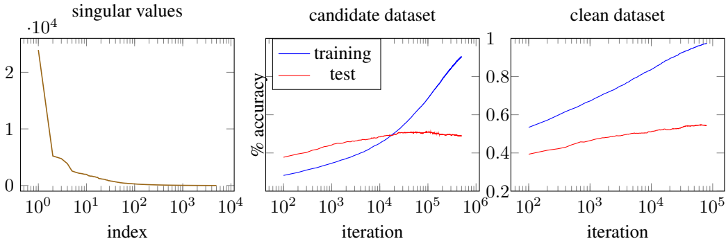
Figure 6: Training a large random feature model on a subset of our candidate training set (middle) and the CIFAR-10 training set (right) with gradient descent. Singular values of the feature matrix (left) shows the low-rank structure for our candidate training set.
