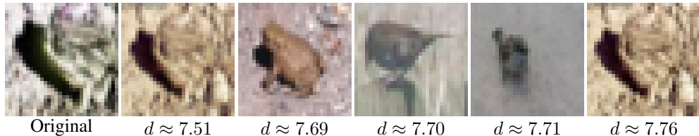
Figure 8: Top-5 closest images to an test image in \ell_2 -distance ( d ). The image at distance d = 7.76 is almost equal to the original one, while a closer one, at d = 7.69 is a different image.
