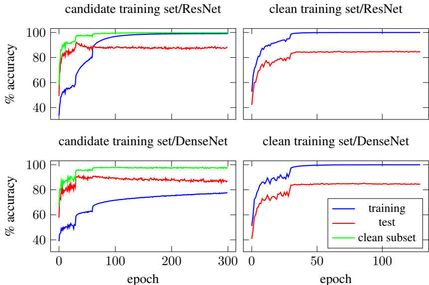
Figure 2: Accuracy on the training set, test set throughout training of the ResNet-18 and DenseNet-110 ( k=12 ) models on our training set (left) and original CIFAR-10 training set (right). For the experiment on our training set, we also show the accuracy on a subset of the training set that is known to have clean labels and corresponds to CIFAR-10 test set.
