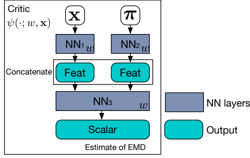
Figure 4: A brief example of the critic in EMD.
