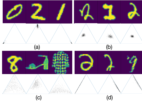
Figure 2: An empirical example of MC estimate of the induced distribution over simplex. The classifier (MCDP) is trained on real-world digits images of \{0, 1, 2\} (corresponding to left, right, top corners of simplex). The 1st and 3rd rows indicate the input while the 2nd and 4th rows indicate MC estimate of \pi over a 2-simplex.
