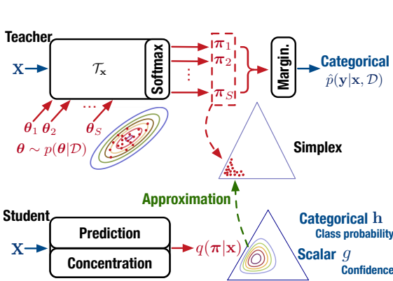
Figure 1: An intuitive example of the proposed framework. Only one input x is considered in this example. “Margin.” indicates marginalization over \pi .
