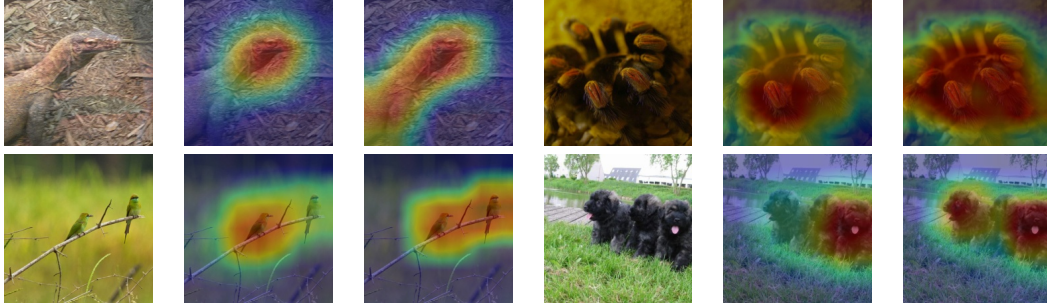
Figure 5: Class Activation Maps (CAM) at the last layer for ResNet-101 (2nd and 5th column) and ResNet-101 with C3 block (3rd and 6th column).
