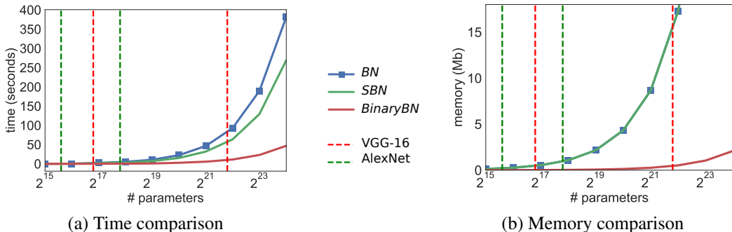
Figure 3: Comparison between time and memory consumption of BN, SBN and BinaryBN for an input feature map of 256 \times 256 . For reference, dotted lines show the minimum and maximum number of parameters that can be found in the BN layers of a VGG-16 network and an AlexNet network.
