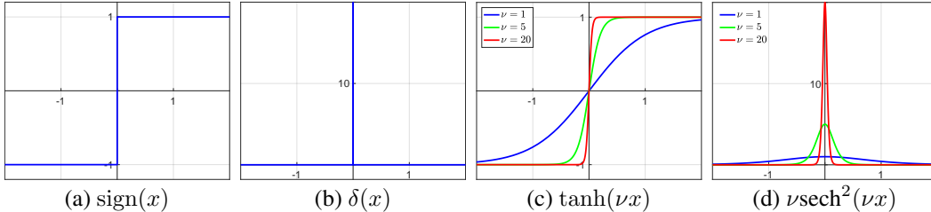
Figure 2: The discrete sign (a) and its derivative (b) are shown. (c, d) show that as \nu takes values of 1, 5, and 20, the scaled tanh converges toward the original sign function and its derivative.
