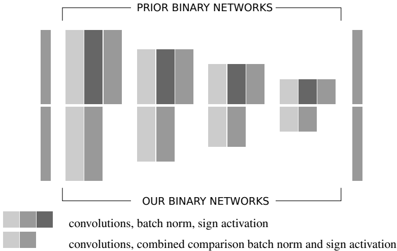
Figure 1: Schematic comparison of a typical binary neural network generated by existing methods (top half) with that of our method (bottom half). Existing methods are unable to avoid the 32-bit floating point batch norm, while we simplify it to a comparison operation, which simultaneously serves as the activation layer.
