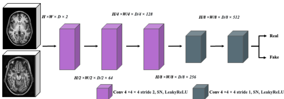
Figure A.3: Discriminator structure.
