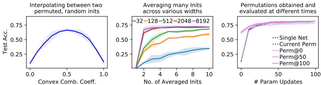
Figure 3: Permutations found after training project random initialisations to same loss valley. Left: Network with two hidden layers of 2048 neurons each, trained on Fashion MNIST. Left- and rightmost point correspond to two random initialisations. The average of the two permutations performs significantly above chance, demonstrating that, after the permutation, the initialisations lie in the same loss valley. Mid: Networks with one hidden layer and different widths. For n > 2 networks, all networks are permuted to be similar to the first network, and then averaged with equal weights. Averaging increasing numbers of random initialisations gradually improves performance. Right: Same architecture as left panel, but permutations are computed and applied at different points at training. We match, permute and average the activations after each parameter update (“Current Perm”, dashed blue). Additionally we apply the permutations found after 0, 50 respectively 100 parameter updates at different times in training (“Perm@x”, shades of pink). Permutations that reveal that initialisations live in the same loss valley can also be found without training the networks, see Appendix B.
