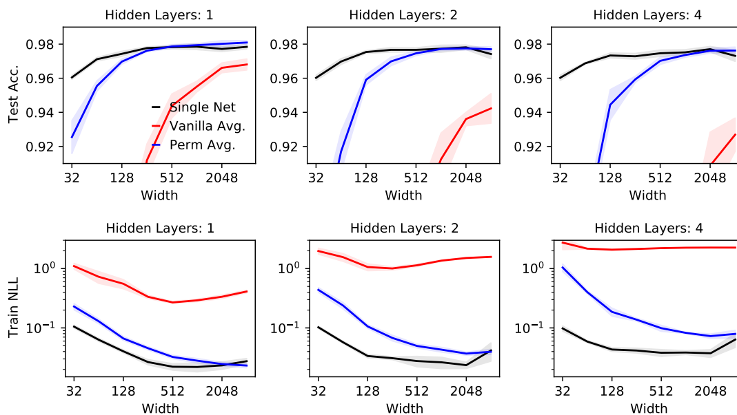
Figure 7: Analogous to Figure 2, but on MNIST. Loss increases at very high width, because in this case lower learning rates would be optimal, but we stick to AdamW default settings.
