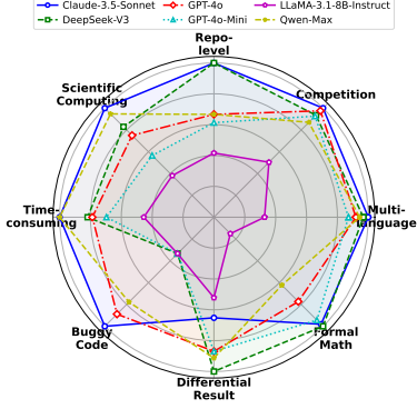
Figure 1: Performance of 6 typical models on SURGE.
