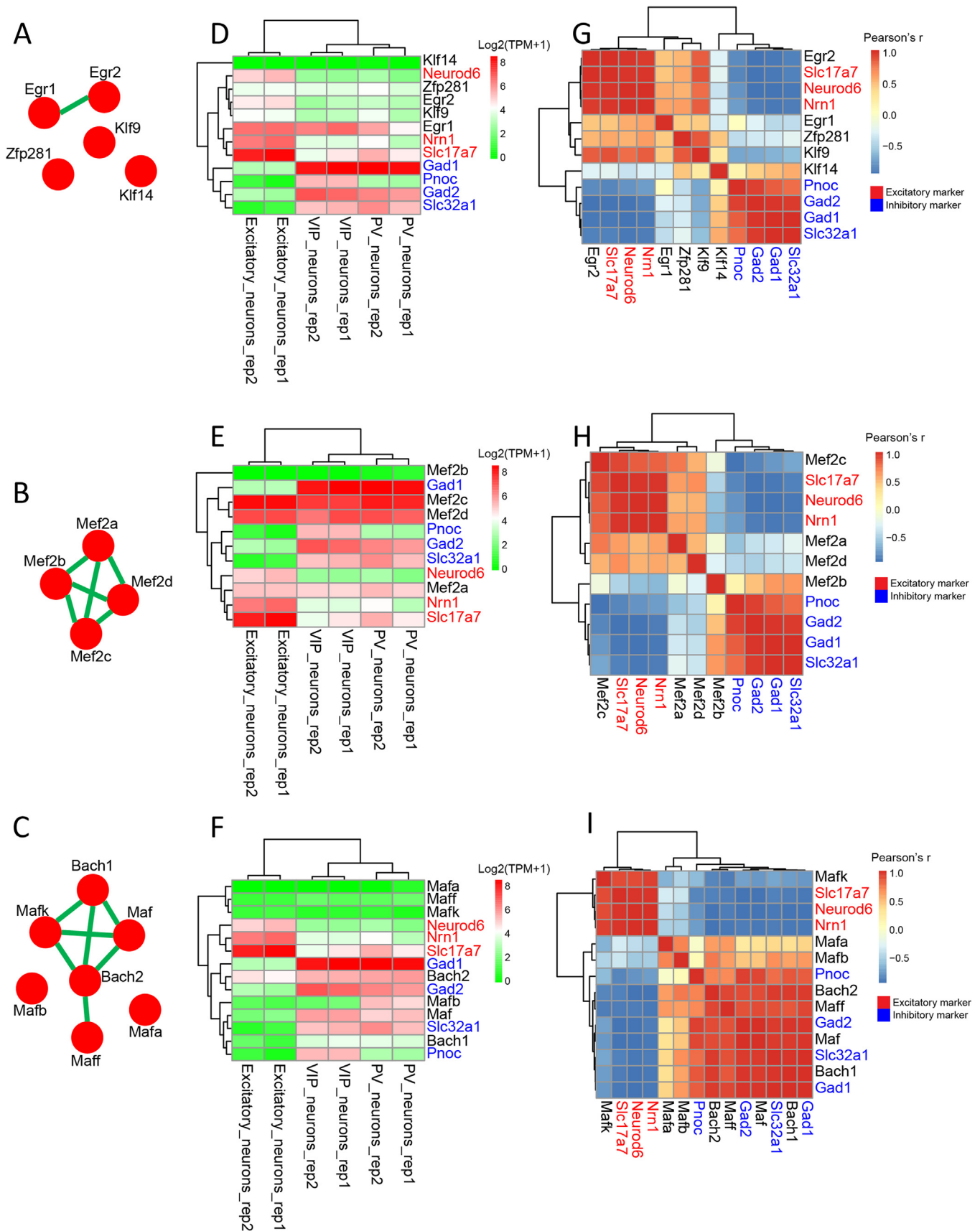
Fig. 4. ETRMs of Egr1 in mPv, Mef2c in mPv, and Maf in mPv. A) ETRM predicted from Egr1 motif in DMRs of mPv neurons. The green edge means that there is evidence in the STRING database to support interaction between the proteins coding from the connected two genes. B) ETRM predicted from the Mef2c motif in DMRs of mPv neurons. C) ETRM predicted from the Maf motif in DMRs of mPv neurons. D-F) Expression of Egr1 ETRM (D), Mef2c ETRM (E), and Maf ETRM (F) in EXC, PV, and VIP neurons. G-I) Correlation between the expression of Egr1 ETRM (G), Mef2c ETRM (H), Maf ETRM (I) and excitatory/inhibitory markers in EXC, PV, and VIP neurons. (For interpretation of the references to color in this figure legend, the reader is referred to the web version of this article.)
