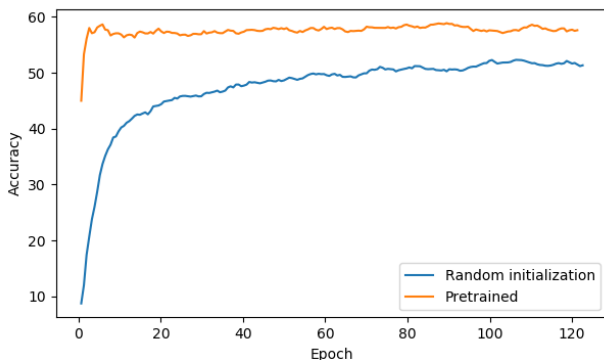
Figure 3: Action recognition results on validation set. This figure shows the accuracy of each method on validation set during the training time.
