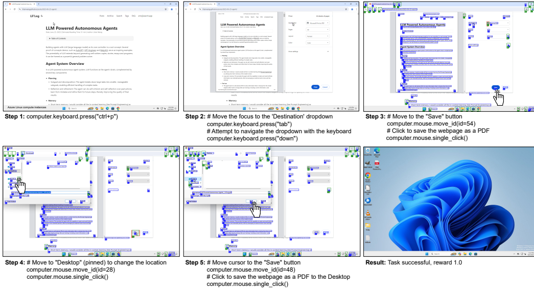
Figure 4: Example of a successful episode in WINDOWSAGENTARENA using a combination of UIA and proprietary models for screen parsing. The agent interacts with mouse and keyboard functions to save a webpage PDF in the desktop.
