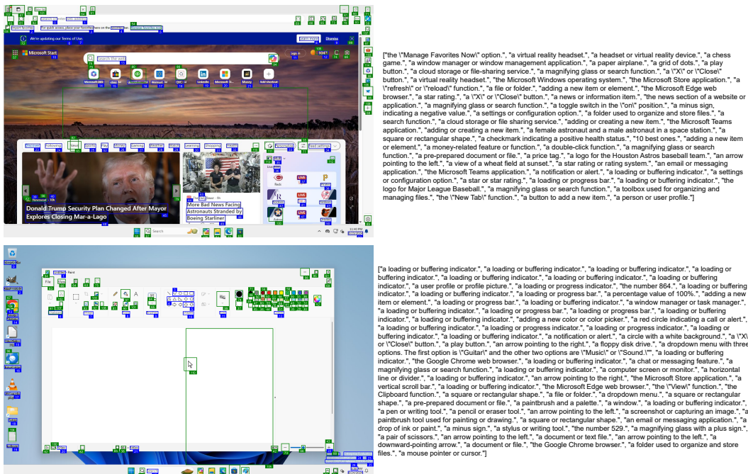
Figure 10: Multiple examples of Set-of-Marks based on Omniparser with text (blue) and icons (green), along with icon captions.
