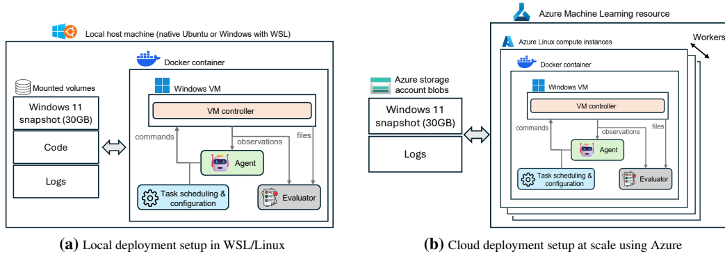
Figure 12: Comparison between local and cloud deployment of WINDOWSAGENTARENA. The benchmark is designed for small scale local testing and large scale cloud parallelization.
