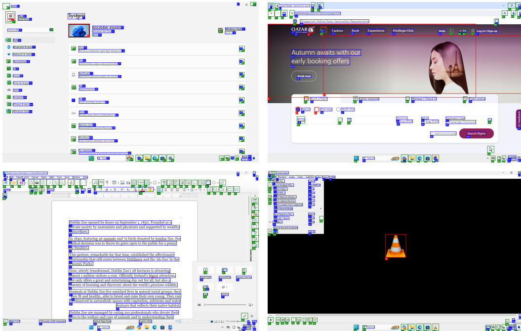
Figure 7: Multiple examples of Set-of-Marks based on proprietary pixel-based local models. OCR (blue), icon detection (green), and image detection (red).
