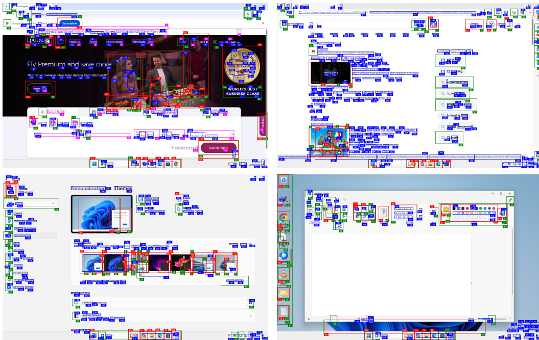
Figure 8: Multiple examples of Set-of-Marks based on open-sourced pixel-based local models. OCR (blue), icon detection (green), image detection (red), and DOM parser (magenta).
