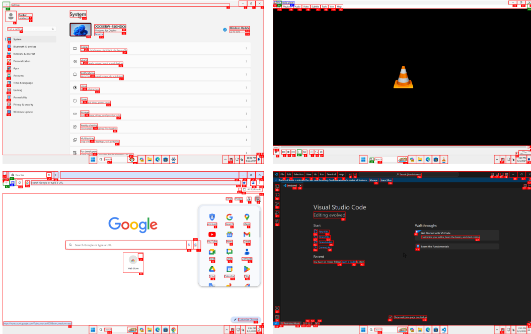
Figure 9: Multiple examples of Set-of-Marks based on UIA tree parser (red).
