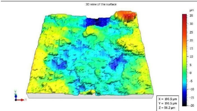
Fig. 5. 3D view of an image taken by a 3D non contact profilometer
