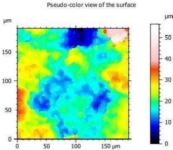
Fig. 4. 2D view of an image taken by a 3D non contact profilometer
