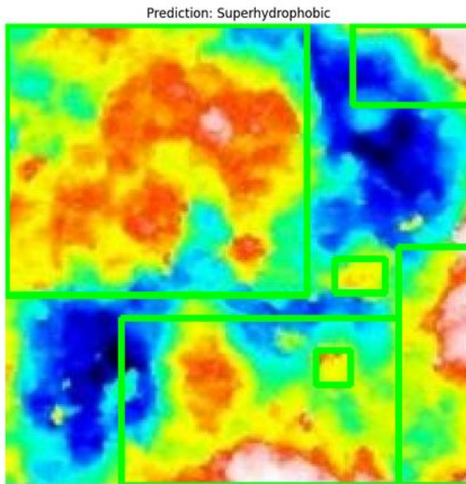
Fig. 9. Bounding box of superhydrophobic 2D view image around red and yellow regions for higher surface roughness detection
