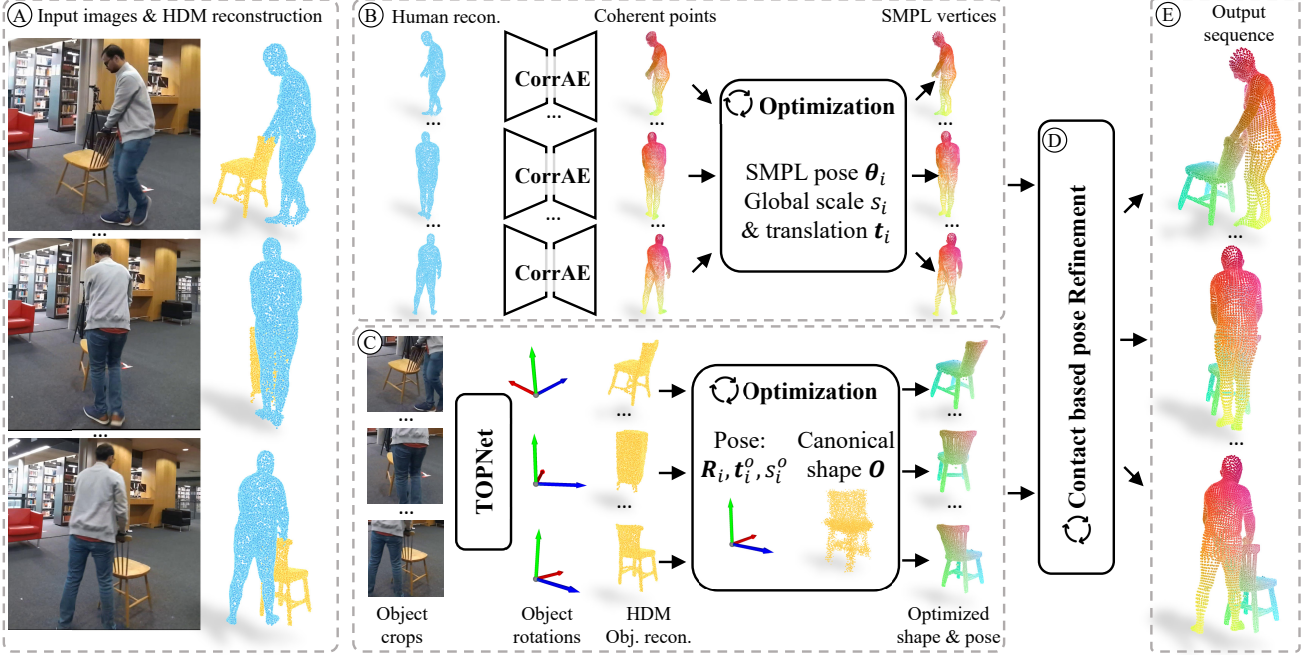
Figure 2. Method Overview. Given an image sequence of human object interaction and HDM [79] reconstructions (A), we aim at obtaining coherent tracking of the human and object across frames (E). We first use a simple yet efficient autoencoder CorrAE to obtain coherent humans points and optimize human via the SMPL layer (B, Sec. 3.2). We then use a temporal object pose estimator TOPNet to predict the object rotation, which allows us to optimize a common object shape in canonical space and fine tune pose predictions (C, Sec. 3.3). We then jointly optimize human and object based on contacts to obtain consistent tracking (D, Sec. 3.4).
