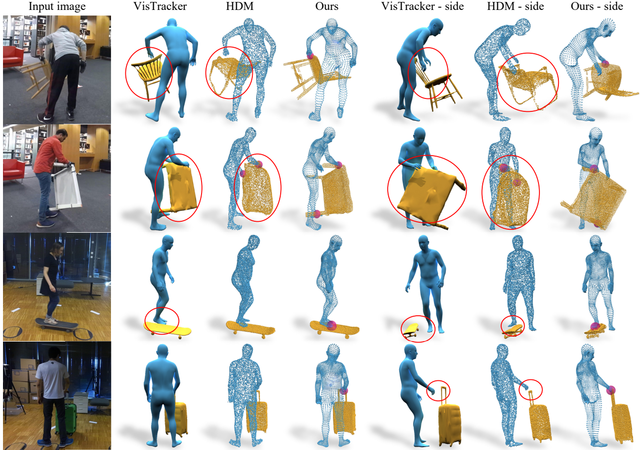
Figure 3. Comparing our method against VisTracker [78] and HDM [79] on BAHEVE (row 1-2) [6] and InterCap (row 3-4) [27]. VisTracker relies on post-hoc processing to refine object pose which is inaccurate and HDM reconstructs inconsistent object shapes (row 1-2) or interactions (row 3-4). Our temporal based pose estimation and optimization leads to consistent shape and interaction.
