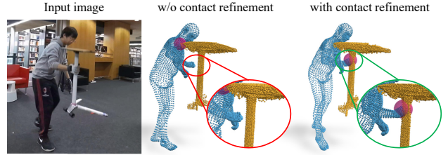
Figure 5. The effect of the contact-based refinement. Without contact, the hand and object can be far apart, leading to implausible interaction.
