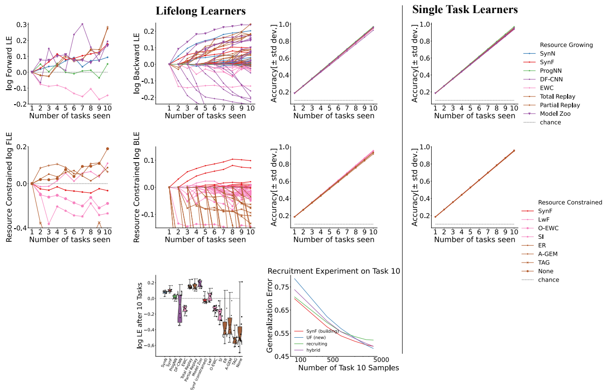
Figure 4: Performance of different algorithms on CIFAR 10x10 vision dataset for 5,000 training samples per task. SYNN maintains approximately the same forward transfer (top left and middle left) and backward transfer (top and middle row second column) efficiency as those for 500 samples per task whereas other algorithms show reduced or nearly unchanged transfer. SYNF still demonstrates positive forward, backward, and final transfer, unlike most of the state-of-the-art algorithms, which demonstrate forgetting. The replay methods, however, do demonstrate transfer, albeit with significantly higher computational cost.
