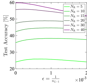
Figure S2: Test accuracy for N_E = 10000 MNIST test data as a function of the inverse width \epsilon = 1/n_{L-1} of the hidden layer with quadratic activation. For each number N_R of subsampled training data, the result is averaged over 10 distinct choices of such subsamplings. For small numbers of training data, finite widths result in regularization effects, improving the test accuracy.
