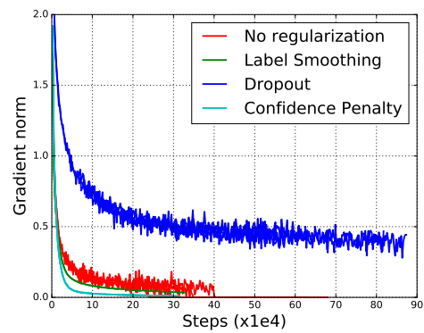
Figure 1: Norm of the gradient as training proceeds on the MNIST dataset. We plot the norm of the gradient while training with confidence penalty, dropout, label smoothing, and without regularization. We use early stopping on the validation set, which explains the difference in training steps between methods. Both confidence penalty and label smoothing result in smaller gradient norm.
