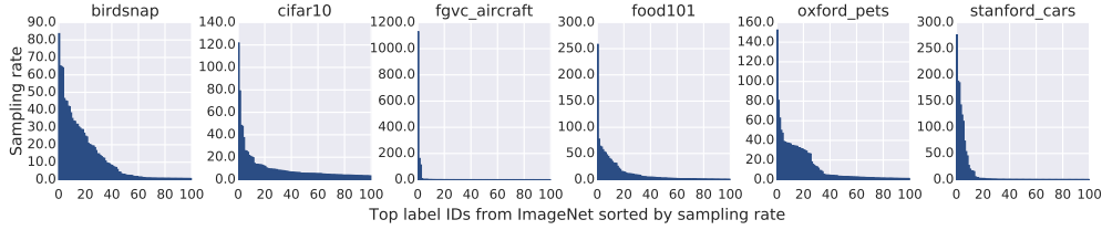
Figure 1: Distribution of importance weights for each target dataset when using ImageNet as a source pre-training dataset. The horizontal axis represents the top 100 ImageNet labels sorted by importance weight for each dataset; each dataset has a different order. The distributions vary widely between target datasets. FGVC Aircraft selects only a few labels that turn out to be coarse grained, whereas Oxford Pets selects a wider variety of fine-grained labels. This reflects the inherent bias in the ImageNet dataset.
