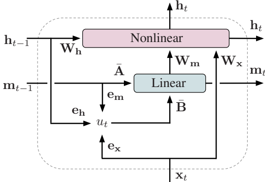
Figure 2: Time-unrolled LMU layer. An n -dimensional state-vector ( \mathbf{h}_t ) is dynamically coupled with a d -dimensional memory vector ( \mathbf{m}_t ). The memory represents a sliding window of u_t , projected onto the first d Legendre polynomials.
