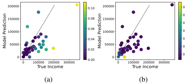
Figure 3: Plots of individuals in an optimization instance in the income regression task, from the perspective of worst-case distributions w.r.t. mse (a) and the utility-based metric (b). The underlying predictive model was trained with mean-squared error loss. For each worst-case distribution, we display over all individuals their model predictions, label income, and assigned weights. In each figure the identity line (True Income = Model Prediction) is marked with a dotted line.
