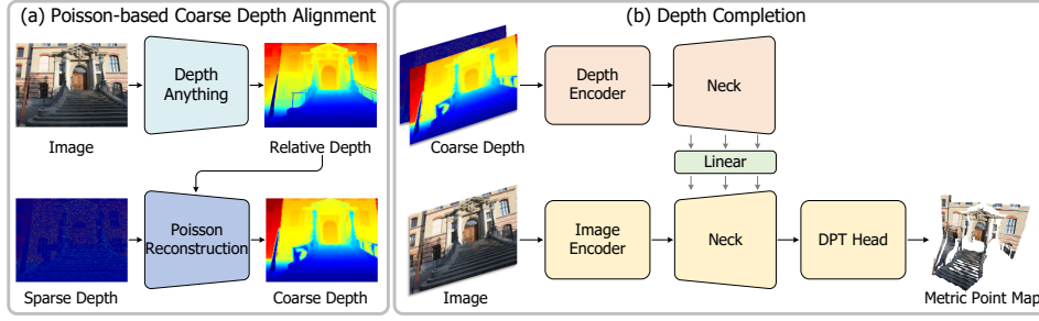
Figure 2: Schematics and detailed architecture of LDCM. Given a single image and sparse depth map, LDCM begins with a Poisson-based coarse depth alignment strategy. This process leverages a pretrained depth foundation model to generate an initial coarse depth map through gradient-domain optimization. This coarse depth, together with the input image, is then fed into the following point map prediction network to regress a dense, metric-scale 3D point map.
