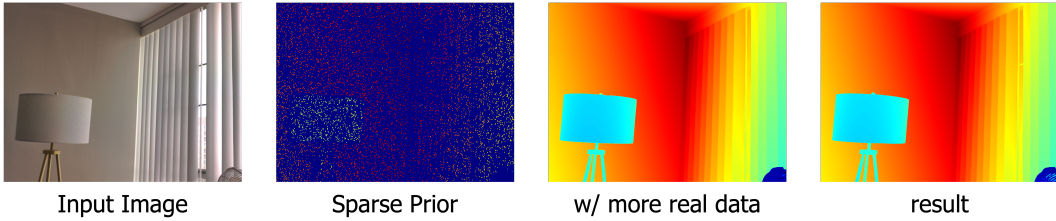
Figure 5: Qualitative comparison between the results from models using different training datasets.
