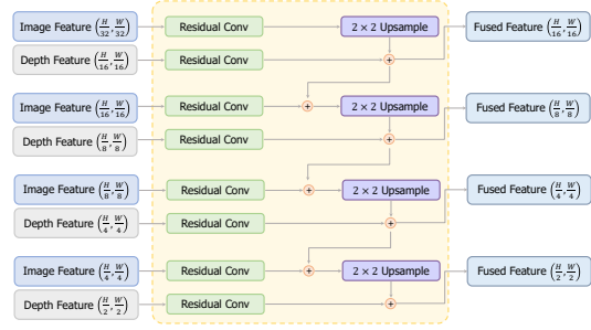
Figure 3: Detailed structure of the image neck.
