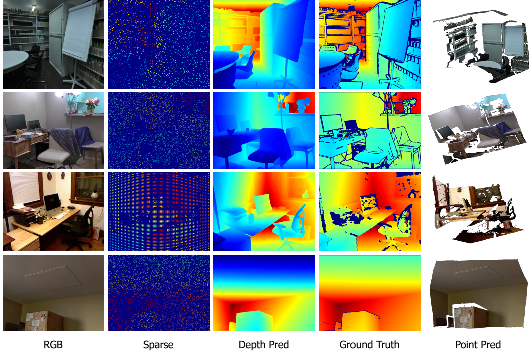
Figure 9: More visualization results for depth map and point map.
