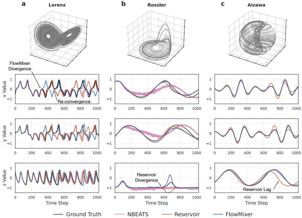
Figure 3: Predictions of Lorenz (a), Rössler (b), and Aizawa (c) chaotic attractors (scaled [-1,1]). Each row shows the evolution of x, y, and z variables over time. Ground truth (black), FlowMixer (blue), Reservoir Computing (orange) [1, 52, 53], and N-BEATS (purple) [32] trajectories are compared. While all methods capture the Lorenz attractor’s structure, N-BEATS shows a notable deviation in the Rössler system, and Reservoir Computing shows differences particularly in the z-component predictions. FlowMixer exhibits consistent performance across all three systems. Experimental settings are summarized in Appendix C and presented in detail in Appendix K.4.
