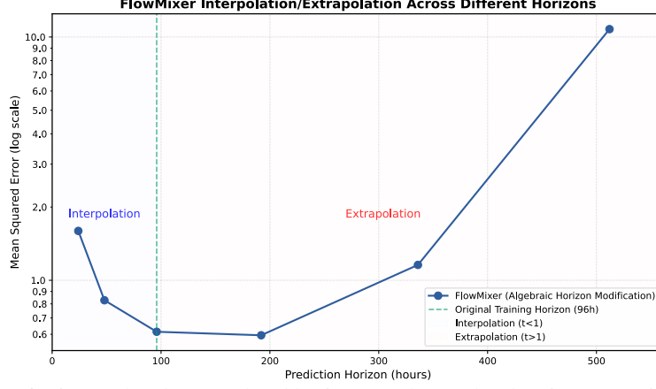
Figure 10: MSE for interpolated/extrapolated horizons on log scale, showing approximately exponential error growth for large deviations from the training horizon.
