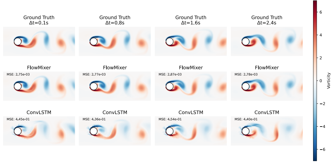
Figure 16: Comparison of vorticity field predictions for 2D flow past a cylinder at Re=150 . The figure shows predictions at four time points ( \Delta t = 0.1s, 0.8s, 1.6s , and 2.4s ) for ground truth, FlowMixer, and ConvLSTM. FlowMixer demonstrates strong performance in capturing the complex vortex shedding patterns, maintaining accuracy over longer time horizons. The color scale represents vorticity magnitude, with red indicating positive (counterclockwise) and blue indicating negative (clockwise) vorticity. Mean Squared Error (MSE) values are provided for each prediction, highlighting FlowMixer's consistently lower error rates than ConvLSTM across all time steps.
