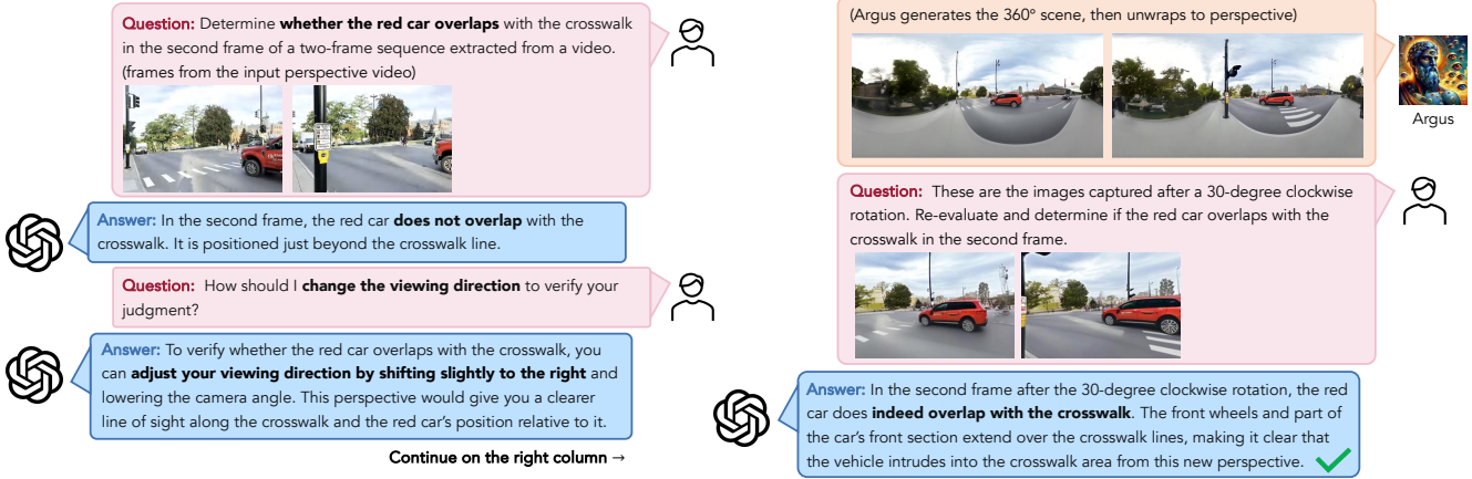
Figure 11. Interactive visual question answering. The first image sequence shows a red vehicle approaching a crosswalk, where the vision-language model (GPT-4o) fails to answer the question correctly because it lacks full scene comprehension. With Argus, we can freely rotate the camera, enabling better spatial understanding and accurately revealing the vehicle’s overlap with the crosswalk.
