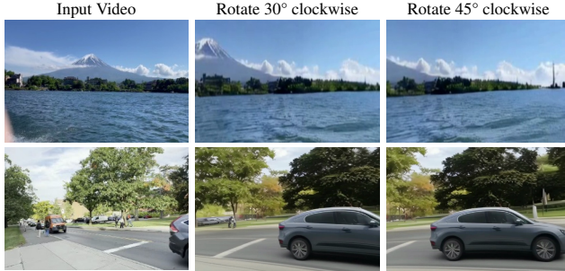
Figure 9. Camera control in dynamic scenes (videos embedded) . Our model enables free camera rotation within dynamic scenes to capture elements beyond the initial viewpoint.
