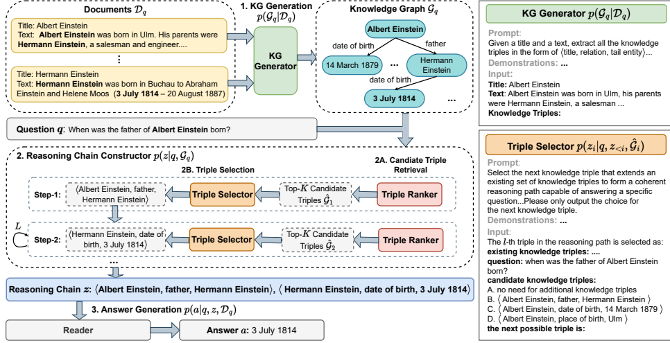
Figure 2: Overview of TRACE. Given a multi-hop question and the retrieved documents, TRACE first uses a KG generator to create a KG based on the documents. It then employs an autoregressive reasoning chain constructor to build reasoning chains from the KG, which are subsequently passed to a reader to generate the answer.
