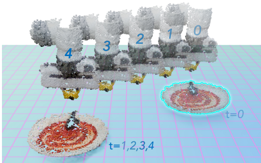
Fig. 9: Illustration for the ADR strategy. Asynchronous transformations are applied to the disturbed object and the robot end-effector to simulate the disturbance resistance process.
