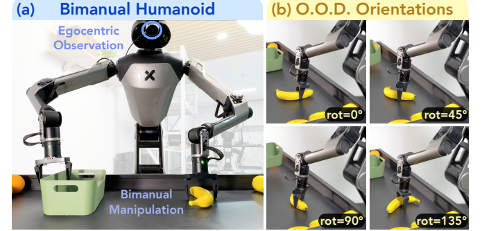
Fig. 5: Bimanual humanoid platform. (a) Egocentric observations and bimanual manipulation. (b) The Fruit-Basket task involves the out-of-distribution orientations during evaluation.
