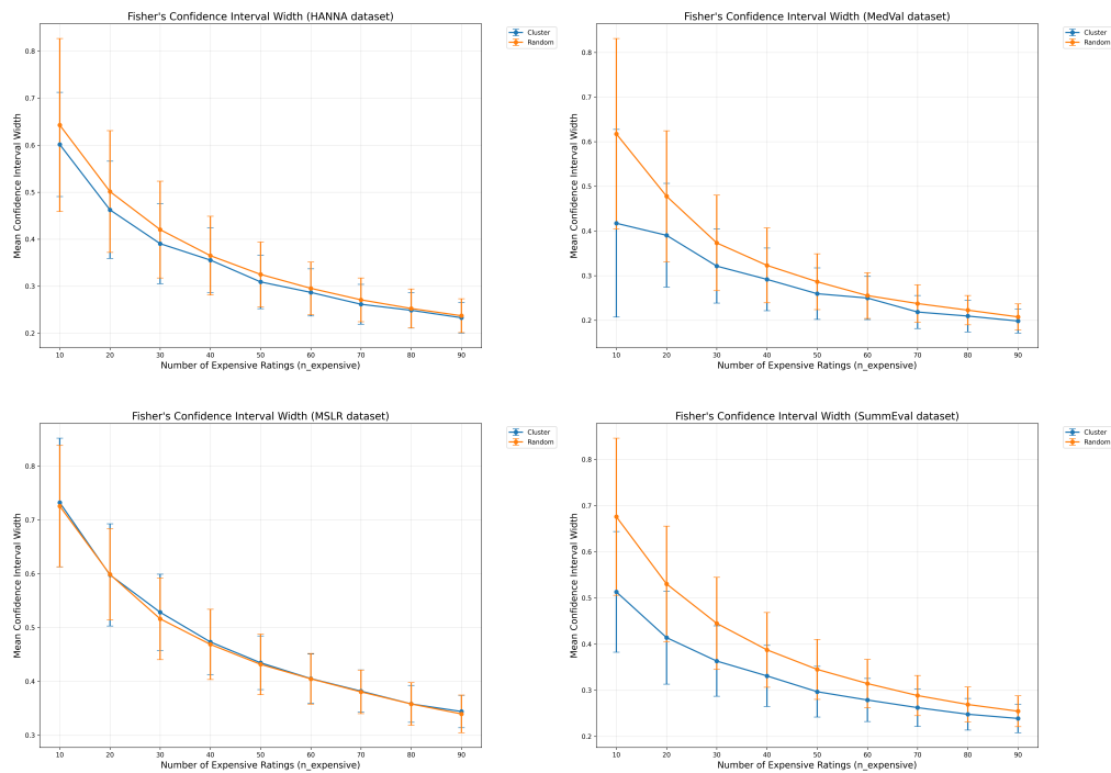
Figure 3: Cluster selection yields more narrow confidence intervals than random selection. 95% confidence intervals for intraclass correlation coefficients (ICC) estimated using the Fisher Z transformation.
