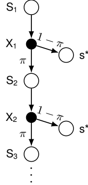
Figure 4: Backup diagram for C-TD ( \lambda ).
