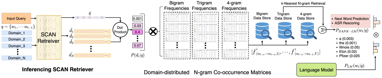
Figure 2: PersonalLM: At inference, we compute the relevance score P(d_i|q) between the query and domains d_i as the dot product of their SCAN retriever representations. We construct a data store for each n-gram frequency matrix. k-most similar n-gram contexts wrt to the input query are retrieved and their weighted summation based on the domain’s relevance score is computed to get probability distribution over targets P_{PersonalLM}(w_t|q) and interpolated with LM probabilities P_{LM}(w_t|q) .
