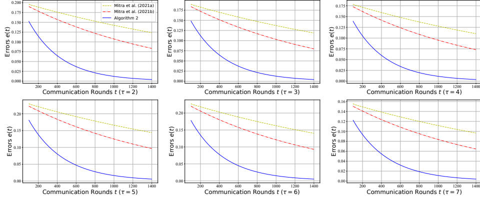
Figure 8: Comparisons of the performance of Algorithm 2 under the proposed stepsize with Mitra et al. (2021a;b) under different local training periods \tau
