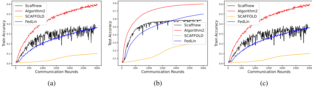
Figure 3: Comparison of Algorithm 2 with state-of-the-art federated learning algorithms—SCAFFOLD, FedLin, and Scaffnew—on the CIFAR-100 dataset. Each curve represents the average of five independent runs. The test accuracy in Figure 2(b) is top-5 accuracy.
