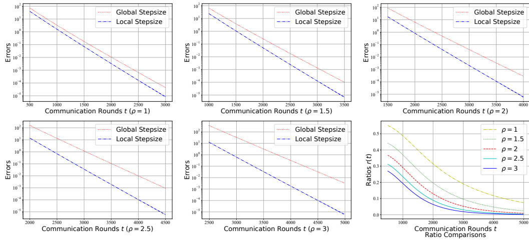
Figure 9: Comparisons of the local stepsize strategy with a universal stepsize strategy under different heterogeneity parameters \rho .
