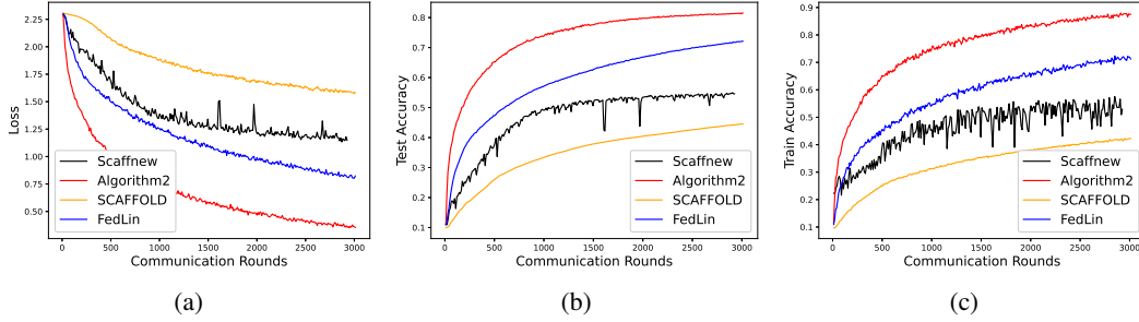
Figure 2: Comparison of Algorithm 2 with state-of-the-art federated learning algorithms—SCAFFOLD, FedLin, and Scaffnew—on the CIFAR-10 dataset. Each curve represents the average of five independent runs.
