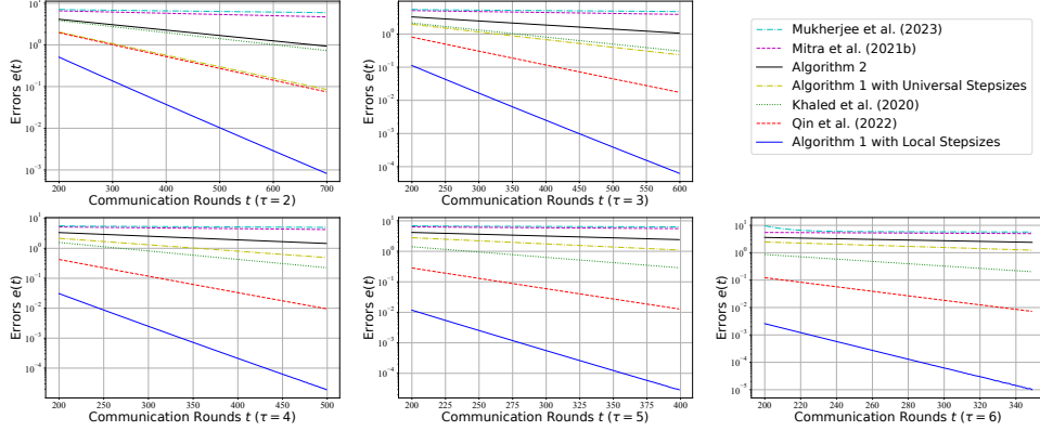
Figure 1: Comparisons of the performance of Algorithm 1 and Algorithm 2 under the proposed stepsize with Qin et al. (2022); Mukherjee et al. (2023); Mitra et al. (2021b); Khaled et al. (2020) under different local training periods \tau .
