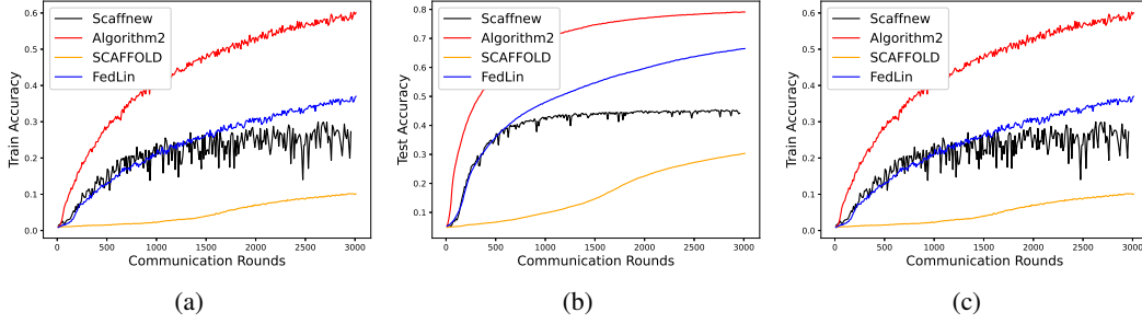
Figure 7: Comparison of Algorithm 2 with state-of-the-art federated learning algorithms—SCAFFOLD, FedLin, and Scaffnew—on the CIFAR-100 dataset. Each curve represents the average of five independent runs. The test accuracy in Figure 2(b) is top-5 accuracy. To induce smaller heterogeneity in data distribution, the Dirichlet distribution parameter was set to \alpha = 10 .
