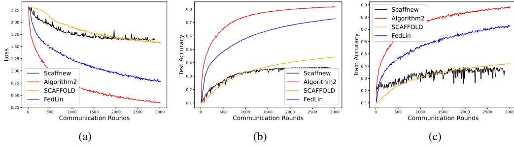
Figure 6: Comparison of Algorithm 2 with state-of-the-art federated learning algorithms—SCAFFOLD, FedLin, and Scaffnew—on the CIFAR-10 dataset. Each curve represents the average of five independent runs. To induce smaller heterogeneity in data distribution, the Dirichlet distribution parameter was set to \alpha = 10 .
