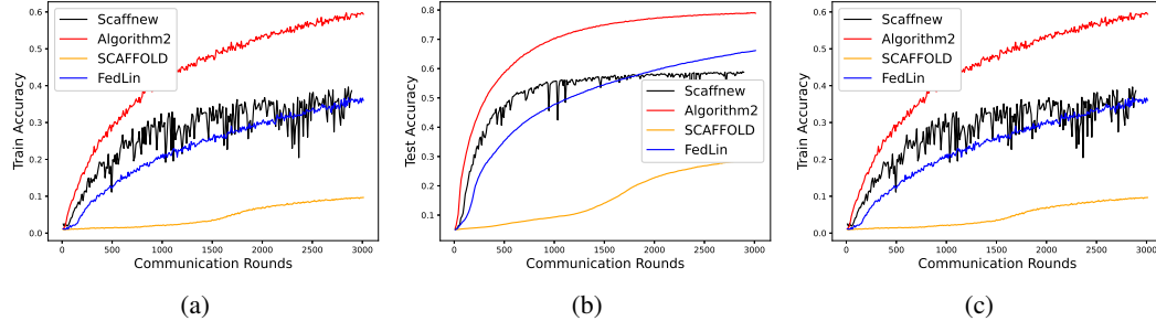
Figure 5: Comparison of Algorithm 2 with state-of-the-art federated learning algorithms—SCAFFOLD, FedLin, and Scaffnew—on the CIFAR-100 dataset. Each curve represents the average of five independent runs. The test accuracy in Figure 2(b) is top-5 accuracy. To induce greater heterogeneity in data distribution, the Dirichlet distribution parameter was set to \alpha = 0.1 .
