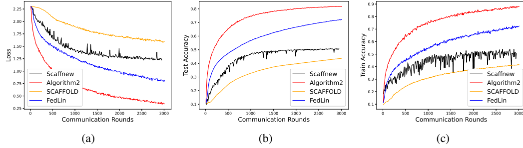
Figure 4: Comparison of Algorithm 2 with state-of-the-art federated learning algorithms—SCAFFOLD, FedLin, and Scaffnew—on the CIFAR-10 dataset. Each curve represents the average of five independent runs. To induce greater heterogeneity in data distribution, the Dirichlet distribution parameter was set to \alpha = 0.1 .
