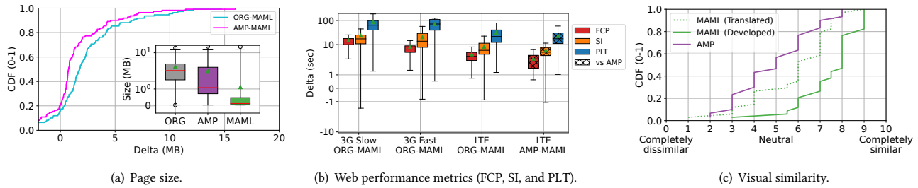
Figure 3: MAML vs. Original (ORG) and AMP in web performance metrics (FCP, SI, PLT), page sizes, and visual similarity.
