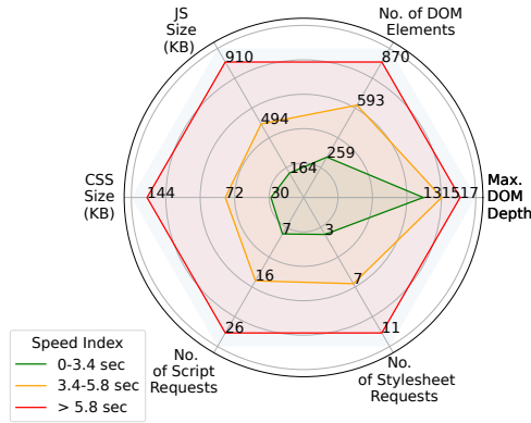
Figure 1: SI versus median complexity metrics as measured via Lighthouse for 100k developing regions websites.
