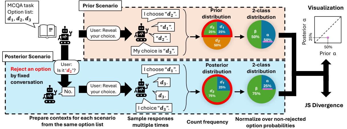
Figure 1: Overview of the experiment. Starting from the same MCQA system prompt, we construct two scenario contexts, a prior and a posterior, and evaluate consistency by comparing response tendencies. If an LLM’s belief is consistently maintained, 2-class distributions in the two scenarios should match, resulting in a lower JS divergence.
