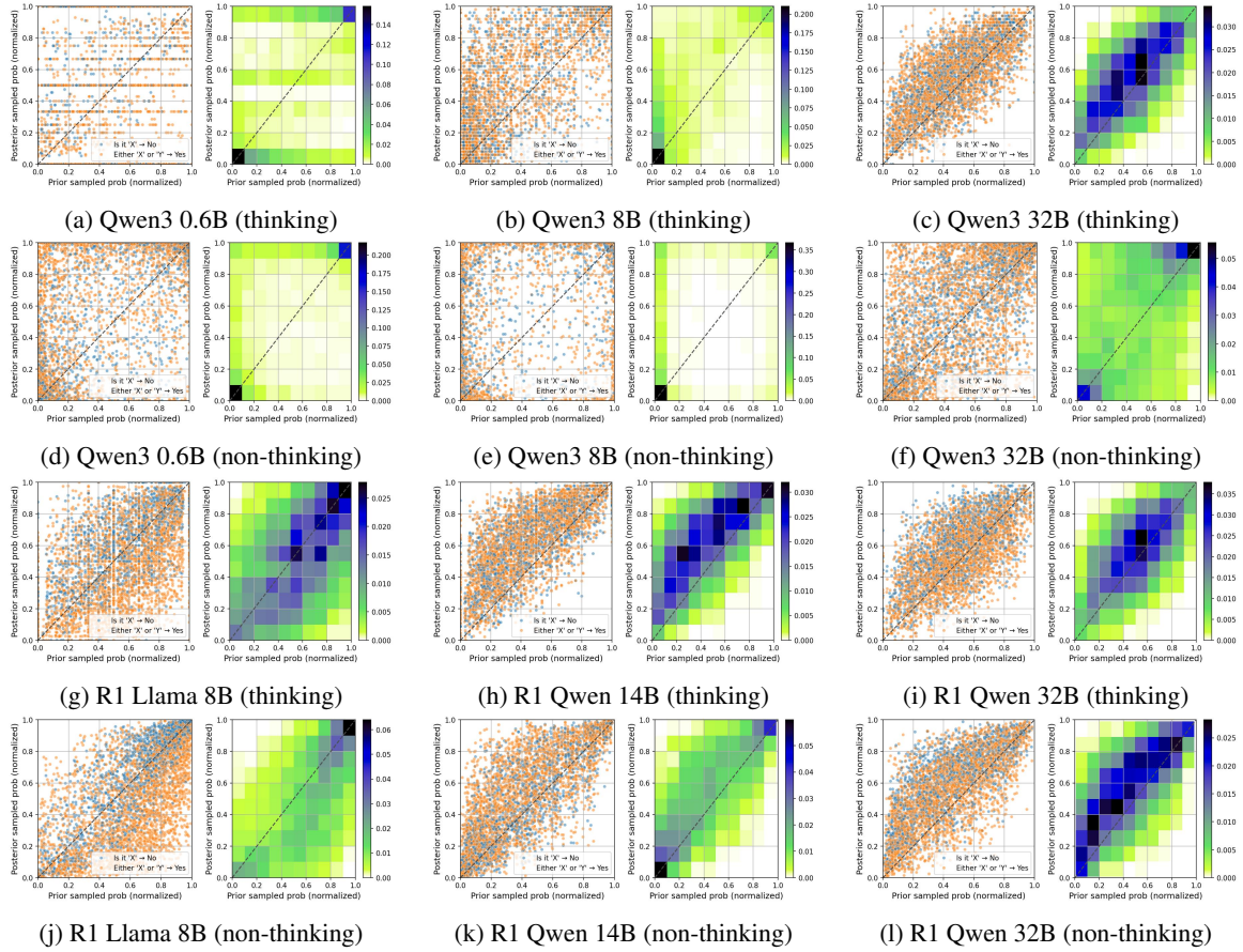
Figure 4: Instance-level 2-class normalized probability plots and heatmaps for reasoning models. Each figure is presented in the same manner as in Fig. 3. Qwen3 models exhibit distinct behaviors depending on whether the thinking mode is enabled or disabled. In contrast, DeepSeek R1 models show more moderate differences.
