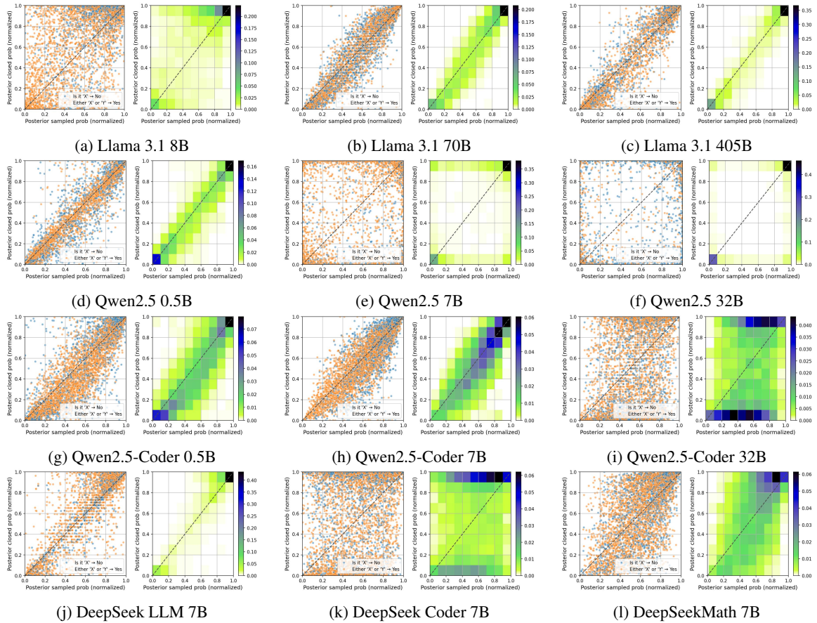
Figure 6: Calibration plots and heatmaps at the posterior context.
