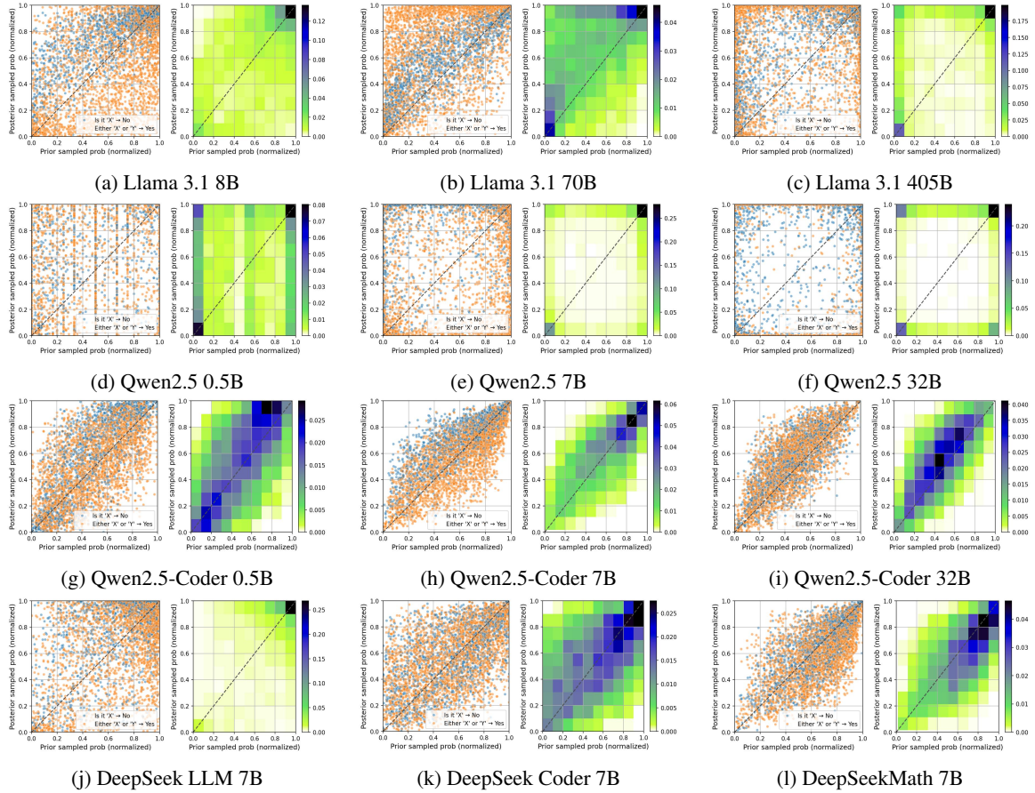
Figure 3: Instance-level 2-class normalized probability plots and heatmaps for non-reasoning models. The horizontal axis represents the normalized probability in the prior scenario for the first not rejected option, p_{\alpha}^{\text{prior}} , and the vertical axis represents the normalized probability in the posterior scenario, p_{\alpha}^{\text{posterior}} , as defined in Equation 2. If consistency holds, the points align along the y = x line. Neither the Llama 3.1 family nor the Qwen2.5 family shows clear improvement with scaling. The Qwen2.5-Coder family exhibits increased entropy and convergence toward the y = x line compared to the corresponding Qwen2.5 models. DeepSeek Coder and DeepSeekMath demonstrate more consistent behavior than the base DeepSeek LLM model.
