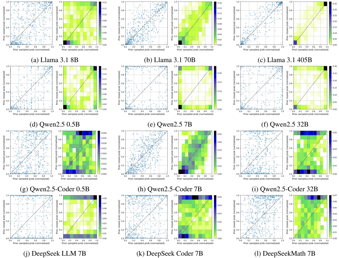
Figure 5: Calibration plots and heatmaps at the prior context.
