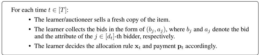
Figure 2: Online Auction with k Attributes.
