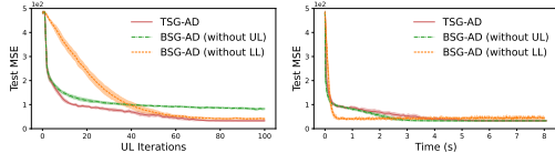
Figure 5: Adversarial learning formulation equation F.18, red wine quality dataset.
