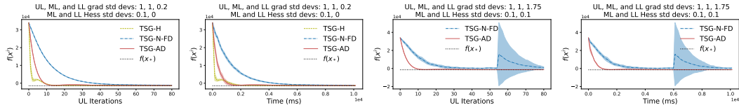
Figure 3: Quadratic problem, stochastic case (low noise: two left plots; high noise: two right plots).
