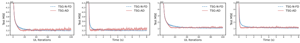
Figure 10: Trilevel adversarial learning formulation proposed in Sato et al. (2021), red wine quality dataset. The two left plots correspond to noise with standard deviation 0, and the two right plots to standard deviation 5.
