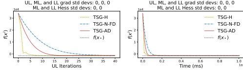
Figure 1: Quadratic problem, deterministic case.
