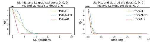
Figure 2: Quartic problem, deterministic case.
