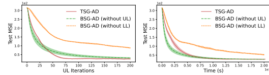
Figure 7: Adversarial learning formulation equation F.18, California housing dataset.
