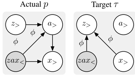
Figure 9: Skill Discovery
