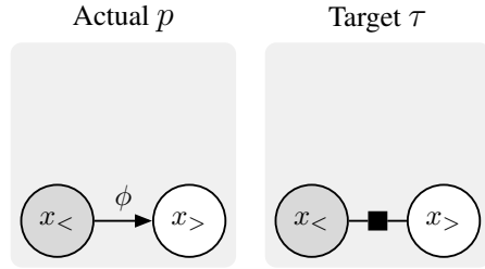
Figure 7: Control
