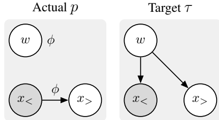
Figure 10: Information Gain
