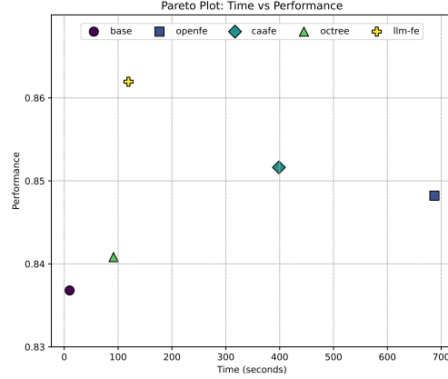
Figure 9: Pareto Plot: comparing trade-off between performance (accuracy) vs time (in seconds) for LLM-FE and other feature engineering baselines.
