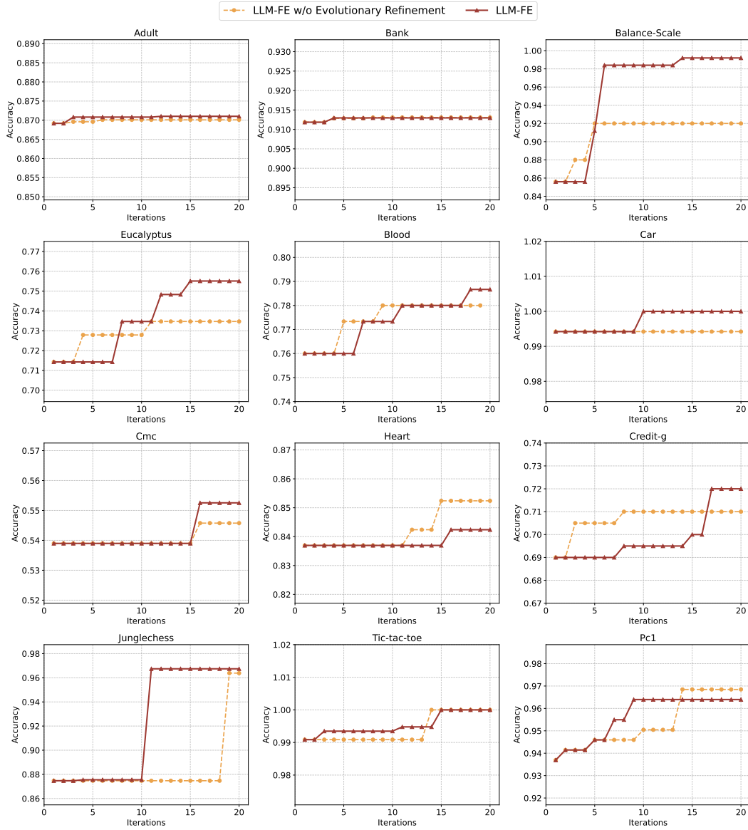
Figure 8: Performance Trajectory Analysis. Validation Accuracy progression for LLM-FE w/o evolutionary refinement and LLM-FE. LLM-FE demonstrates better validation accuracy, highlighting the advantage of evolutionary iterative refinement.
