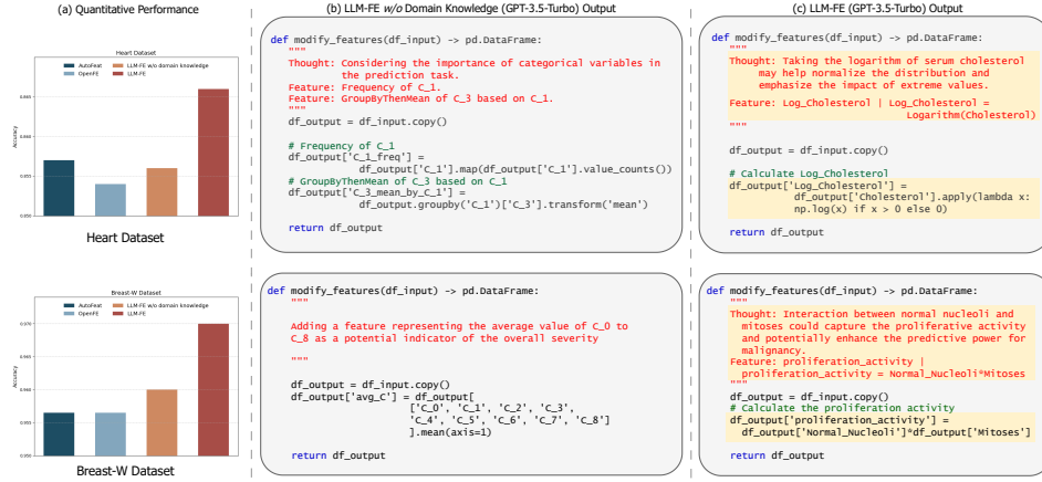
Figure 7: Quantitative and Qualitative Analysis on Impact of Domain Knowledge for LLM-FE on Heart and Breast-W datasets. (a) Comparison of XGBoost performance for LLM-FE against its domain-agnostic variant and traditional methods, such as OpenFE and AutoFeat, which do not integrate domain knowledge and exhibit reduced performance. (b) Features generated using the w/o Domain Knowledge variant of LLM-FE. (c) Feature discovery program generated by LLM-FE. The generated programs emphasize how incorporating domain expertise leads to more interpretable features that improve model performance.
