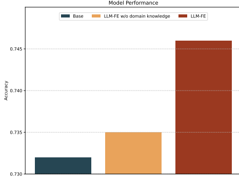
Figure 3: Quantitative impact of domain knowledge on model accuracy. Using domain knowledge boosts performance compared to both the base model and LLM-FE without domain knowledge.
