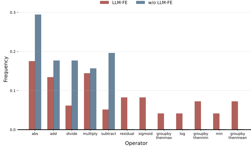
Figure 10: Frequency of Feature Engineering Operators. We compare the operators for LLM-FE with simple LLM-based methods.
