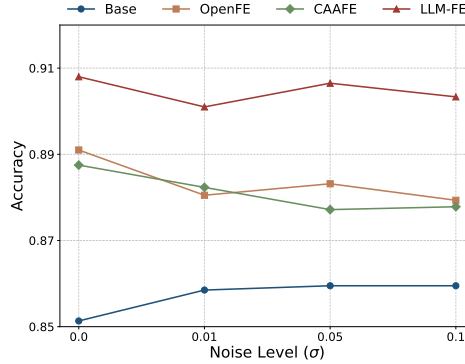
Figure 6: Impact of Noise Levels on XGBoost model performance across different feature engineering approaches, under increasing noise conditions ( \sigma = 0.0 to 0.1 ). We report the mean accuracy across six classification datasets containing only numerical features.
