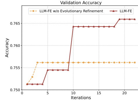
Figure 4: Performance Trajectory Analysis. for LLM-FE w/o evolutionary refinement and LLM-FE. LLM-FE demonstrates a better trajectory, highlighting the advantage of evolutionary refinement.
