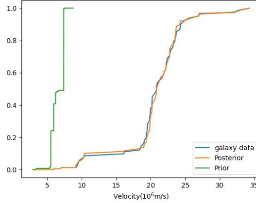
Figure 5: A random measure sampled from DP prior, DP posterior compared against original galaxy dataset distribution.
