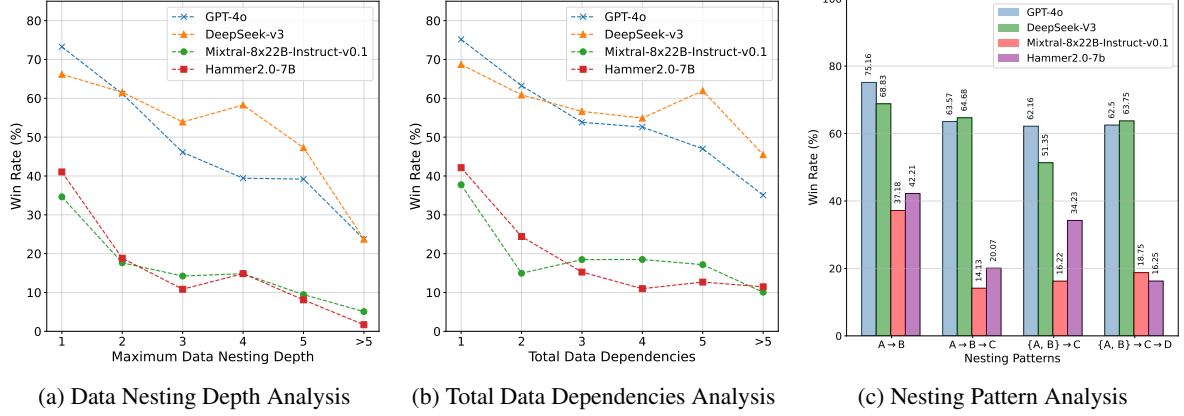
Figure 6: Top 4 models’ performances (on the three-shot setting) with a varying number of (a) longest data dependencies, (b) the total number of data dependencies, and (c) common data nesting patterns in NESTFUL. We observe that models perform well for the simple data samples, however, the performance drops sharply with complicated structural patterns in the data.
