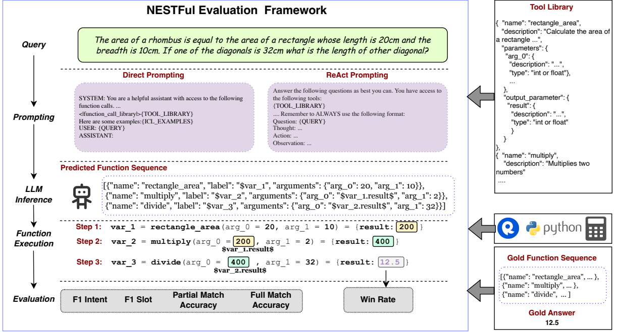
Figure 1: End-to-End Evaluation Pipeline: NESTFUL provides a test set of input queries and its corresponding list of nested function calls. It also provides executable implementations for each tool in the library and allows for evaluating models in direct prompting or REACT styles. Given a query, the pipeline infers the input LLM to generate the required sequence of function calls, execute those functions (taking into account nested variables) and compare the final answer with the gold one.
