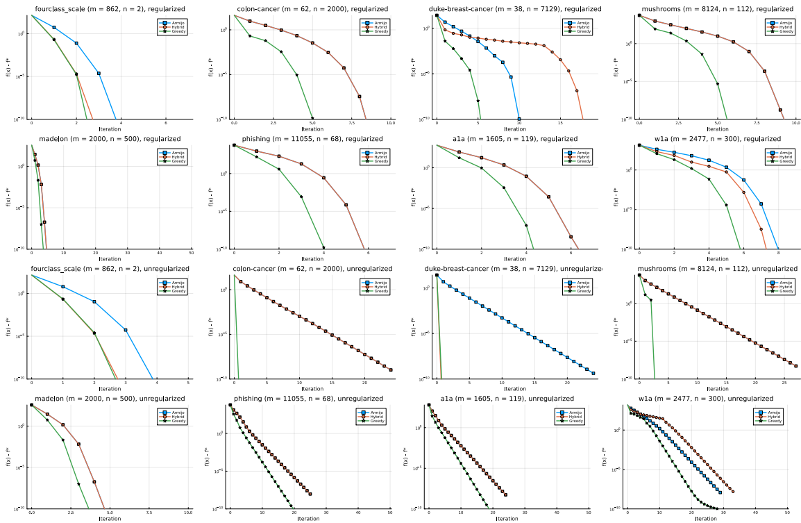
Figure 5: Comparison of methods on real logistic regression datasets, in 8 cases where we observed atypical performance in either the regularized or unregularized setting.
