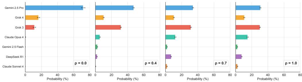
Figure 12: Robust lotteries diversify the lottery to handle preference tradeoffs among ethnic groups in the HUMAINE dataset. We present the estimated probability assigned to each model when annotators are grouped based on ethnic group.
