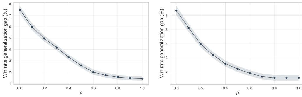
Figure 16: Robust lotteries reduce overfitting in the Search Arena dataset. Groups defined by annotator’s prompt language (Left) and primary intent (Right).
