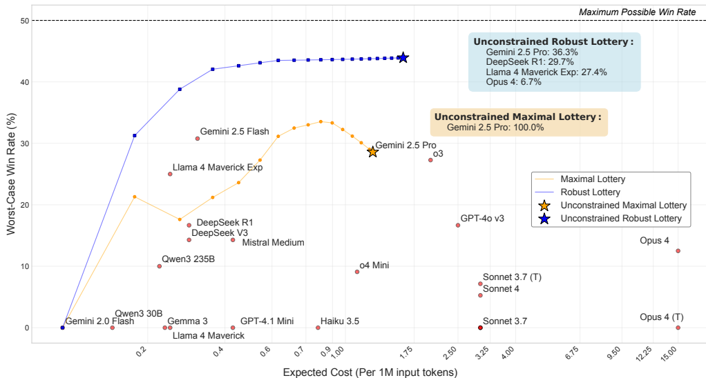
Figure 1: Robust lotteries improve worst-case win rate across user subpopulations. We consider a fixed set of models (red points) and partition the LMArena votes according to the language of the prompt. We then evaluate any lottery (a probability distribution over models) by its worst-case performance on LMArena ( y -axis): the minimum win rate the lottery achieves across the four user subpopulations. Because the guarantee is \min_q \Pr(p \succ q) in a symmetric zero-sum game, it is at most 50%. The x -axis reports the policy’s expected inference cost per 1M input tokens. The orange curve traces the cost–performance frontier obtained by solving for the maximal lottery under an expected-cost budget. The blue curve traces the corresponding frontier for robust lotteries , which instead optimize the worst-case guarantee using a robust linear program. Across budgets, robust lotteries achieve substantially higher worst-case performance than the standard maximal lottery.
