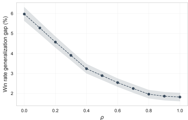
Figure 7: Robust lotteries reduce overfitting in LMArena. We compute robust lotteries for varying radius values \rho and evaluate each lottery on the overall population’s training votes and held-out votes from LMArena. We report the generalization gap (train win rate minus test win rate) as a function of \rho . As \rho increases, the gap shrinks from roughly 6% at \rho = 0 – which corresponds to a standard maximal lottery – to about 2% at \rho = 1 , indicating that robustness regularizes the learned mixture and yields more stable performance.
