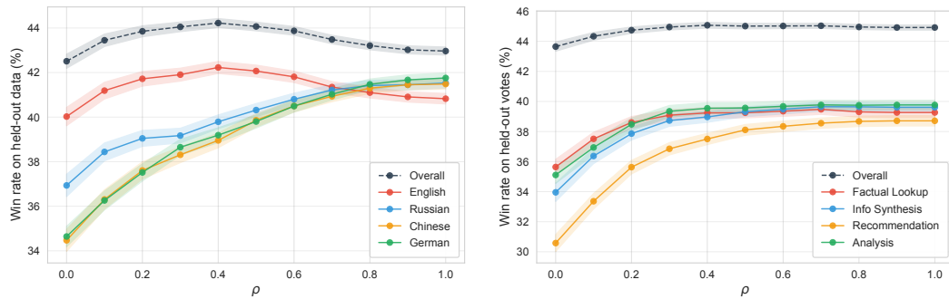
Figure 15: Win rate achieved by robust lottery on held-out votes in the Search Arena dataset. Groups defined by annotator’s prompt language (Left) and primary intent (Right).
