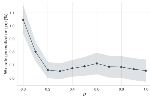
Figure 20: Robust lotteries reduce overfitting in Open LLM. Groups defined by benchmark.
