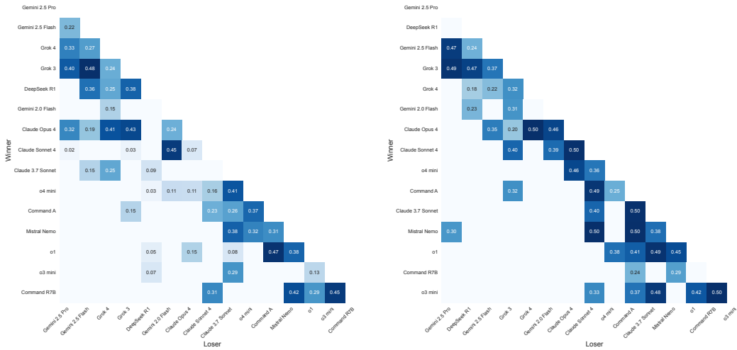
Figure 8: Pairwise preferences exhibit substantial heterogeneity across groups in the HUMAINE dataset. Groups defined by annotator’s ethnic group (Left) and political affiliation (Right).
