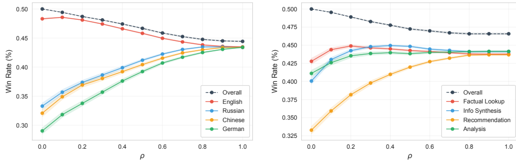
Figure 14: Win rate achieved by robust lottery on training margin matrices in the Search Arena dataset. Groups defined by annotator’s prompt language (Left) and primary intent (Right).
