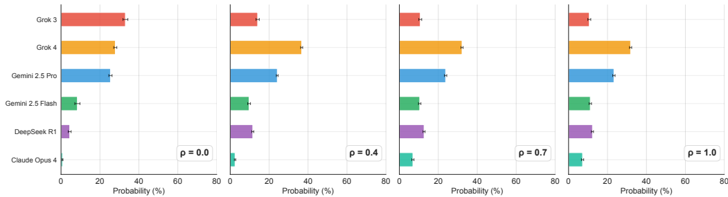
Figure 18: Robust lotteries diversify the lottery to handle preference tradeoffs among tasks in the Search Arena dataset. Groups defined by the annotator’s primary intent in the task.
