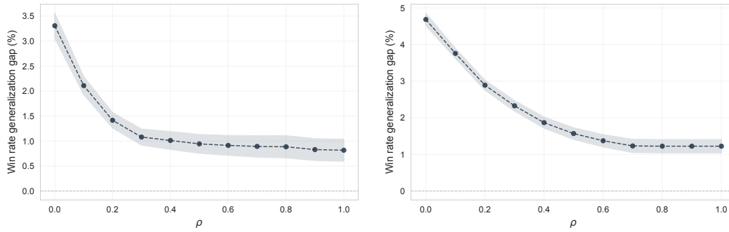
Figure 11: Robust lotteries reduce overfitting in the HUMAINE dataset. Groups defined by annotator’s ethnic group (Left) and political affiliation (Right).
