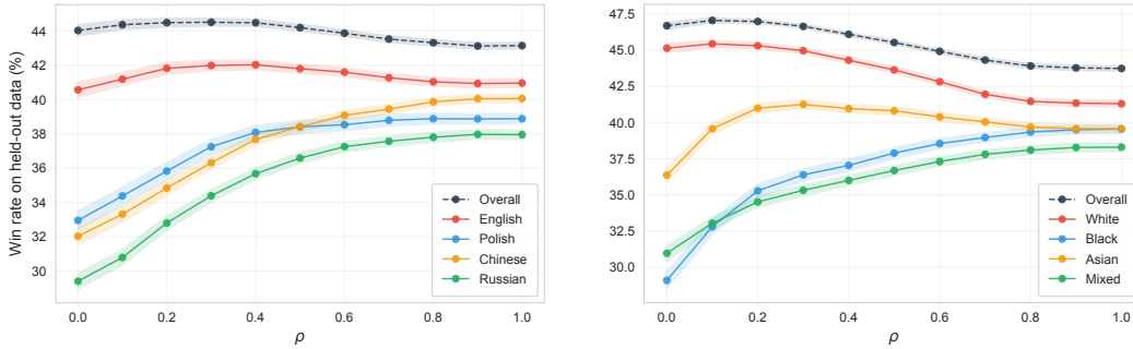
Figure 3: Robust lotteries improve win rate guarantees across user subpopulations. We compute robust lotteries for varying radius values \rho and evaluate each lottery on held-out votes (20% split). We show bootstrap means of win rates achieved on the overall population and each subgroup with standard errors (200 samples). As \rho increases, robust lotteries improve the win rate guarantees for the lowest-performing groups with a modest decrease for the highest-performing groups, illustrating a robustness–accuracy trade-off. Left: LMArena, with groups defined by prompt language. Right: HUMAINE, with groups defined by annotator’s ethnic group.
