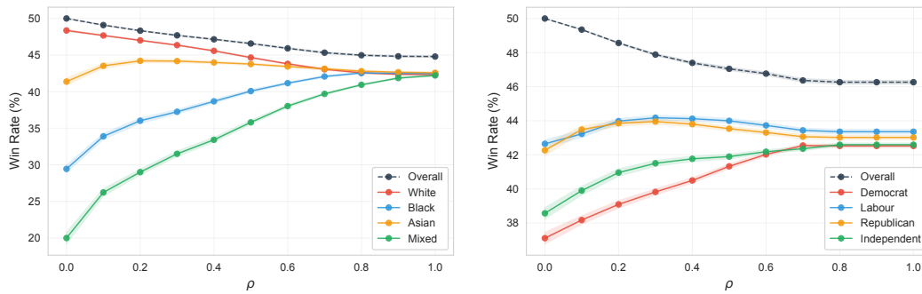
Figure 9: Win rate achieved by robust lottery on training margin matrices in the HUMAINE dataset. Groups defined by annotator’s ethnic group (Left) and political affiliation (Right).
