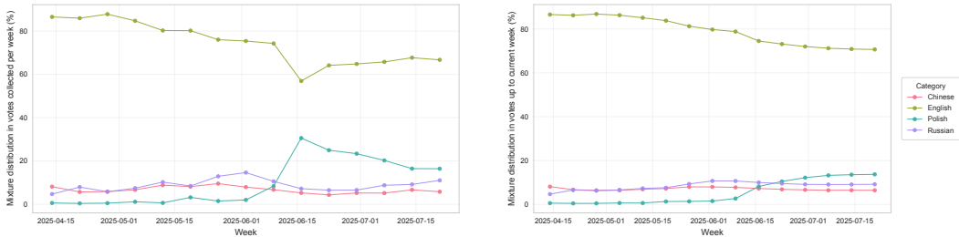
Figure 5: Weekly (left) and cumulative (right) mixture distributions of vote categories in LMArena. The weekly plot shows the fraction of votes collected per category each week, while the cumulative plot shows the category composition of all votes collected up to a given week.
