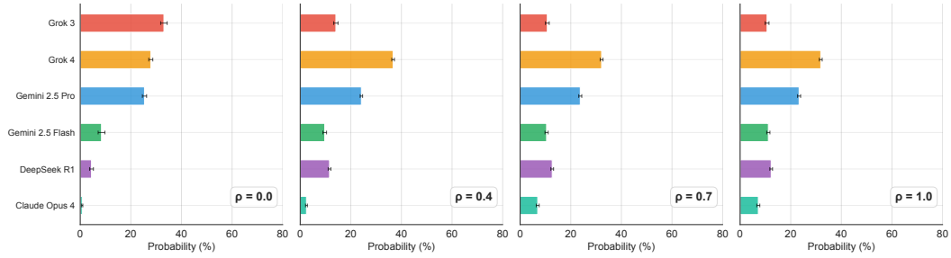
Figure 13: Robust lotteries diversify the lottery to handle preference tradeoffs among political groups in the HUMAINE dataset. Groups defined by political affiliation.
