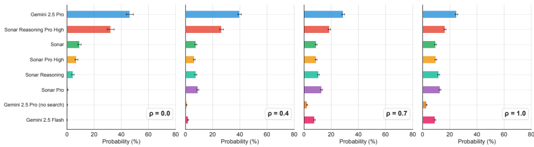
Figure 17: Robust lotteries diversify the lottery to handle preference tradeoffs among languages in the Search Arena dataset. Groups defined by prompt language.
