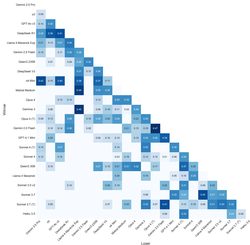
Figure 6: Pairwise preferences exhibit substantial heterogeneity across groups in LMArena. We compute the probability that two distinct groups (sampled proportional to their comparison counts) yield opposite preferences for (i, j) , i.e., their margins M_{ij} have opposite signs.
