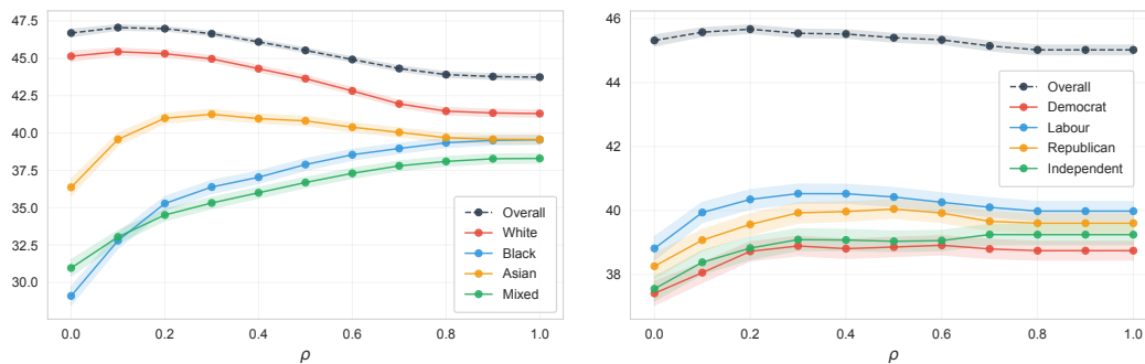
Figure 10: Win rate achieved by robust lottery on held-out votes in the HUMAINE dataset. Groups defined by annotator’s ethnic group (Left) and political affiliation (Right).
