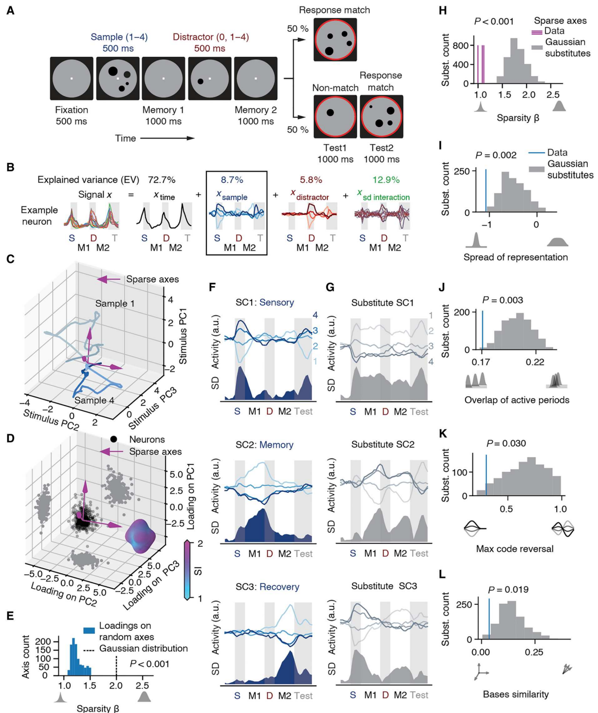
Fig. 2. The neuronal implementation of working memory. (A) Delayed-match-to-numerosity task with distractors. (B) Demixing procedure separating the activity of each neuron into the parts coding time, sample numerosity, distractor numerosity, and sample-distractor interaction. The sample coding part is used for the following analyses. Top: Percentage of explained variance for each part. (C) Representational geometry for sample numerosities 1 and 4 in PC space, averaged across trials of the same condition. (D) Loadings of all recorded neurons on the top three PCs (black dots) including distributions projected onto the planes formed by PC pairs (gray dots). Sparse axes (magenta arrows; determined by SCA) have high SI. Inset: Surface plot of SI for all axes in the space. (E) Sparsity parameter \beta for neuronal loadings on randomly selected axes ( n = 1000 bootstraps) compared to the \beta of a Gaussian distribution. (F) Activity of the three identified SCs, averaged across trials for each sample numerosity condition (top; numbers indicate sample numerosity) and relative information across conditions measured as SD. (G) SCs of an example substitute dataset with nonsparse Gaussian implementation. (H) Sparsity \beta of the neuronal loadings on the SCs for the original data and the substitute datasets (permutation test with n = 3 \times 1000 permutations). (I to L) Activity measures for the SCs of the original data and the substitute datasets (permutation test with n = 1000 permutations). a.u., arbitrary units.
