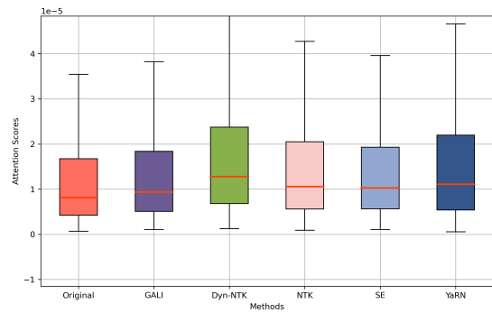
(f) Attention scores of row 6000
