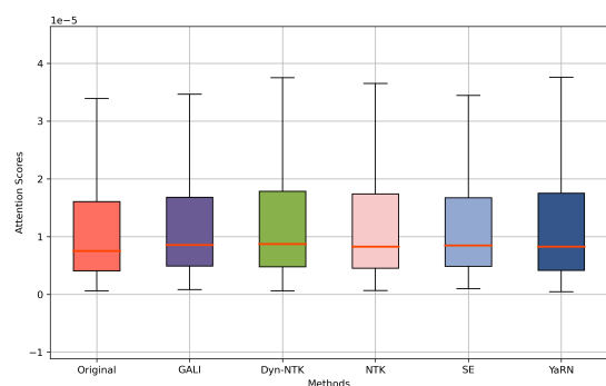
(h) Attention scores of row 8000
