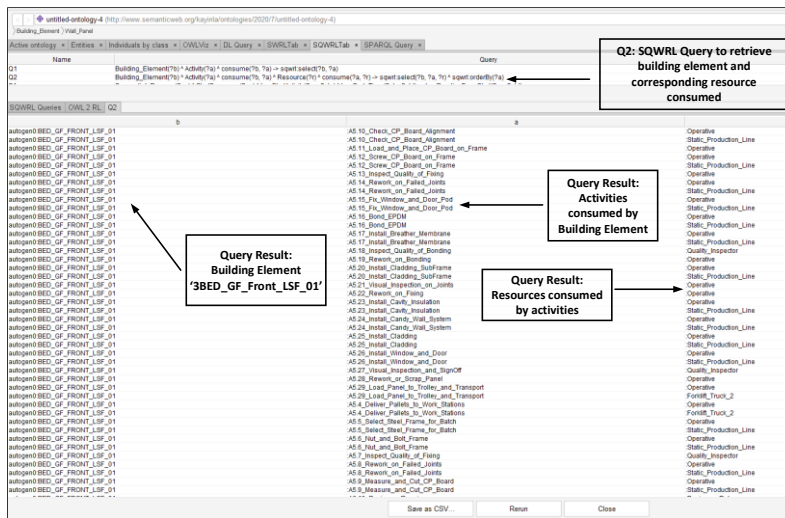
Fig. 6. SPARQL Query Result - Process Information for an instance of wall panel
