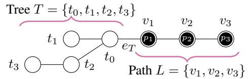
Figure 1: Definition of a shunting tree.
