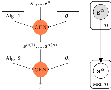
Figure 2: Left: HOM architecture. "Alg. 1/Alg. 2" are Algorithms 1 and 2 respectively. GEN uses \theta_r and \theta_g during evaluation to yield a model which represents the policy. \theta_r and \theta_g are optimized by BO. Right: Inferring \mathbf{a}^\alpha given \mathbf{s}^\alpha .
