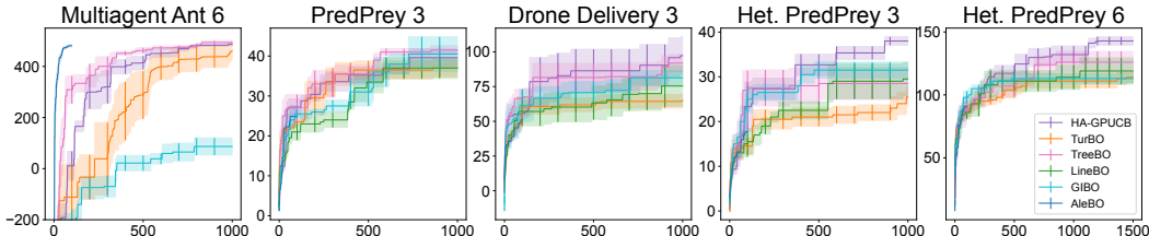
Figure 9: Comparison with BO algorithms. HA-GP-UCB outperforms on complex multi-agent coordination tasks.
