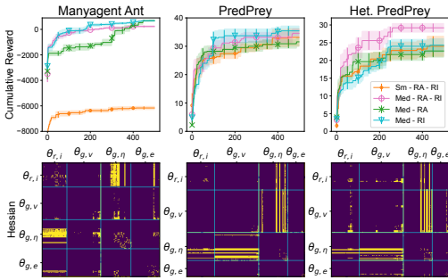
Figure 3: Ablation study. Training curves of our HOM and its ablated variants on different multi-agent environments.
