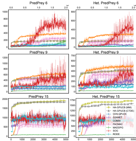
Figure 5: Scaling analysis. Training curves of HA-GPUCB and competitors with increasing number of agents. The left column shows PredPrey with 6, 9, and 15 agents. The right column shows Het, task. Right: Comparison with HDBO approaches. PredPrey with 6, 9, and 15 agents.
