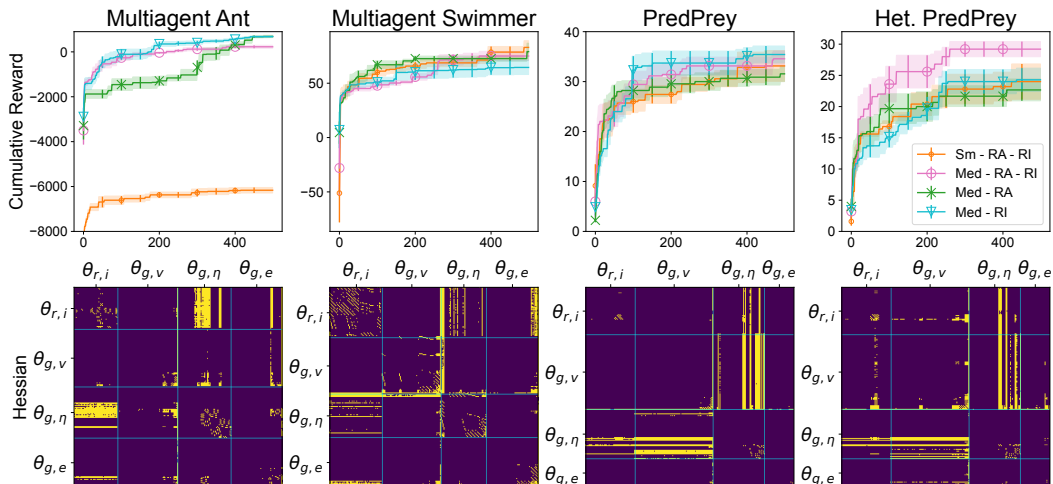
Figure 6: Ablation study. Training curves of HA-GP-UCB and its ablated variants on different multi-agent environments.
