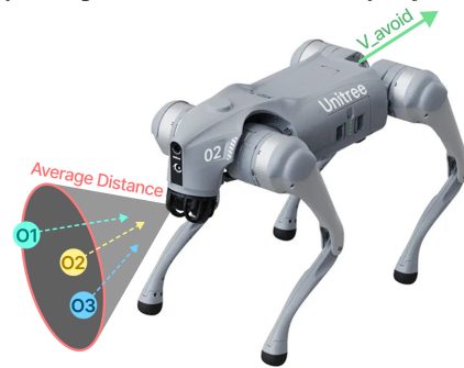
Figure 3: The calculation of the sector-based avoidance velocity.
