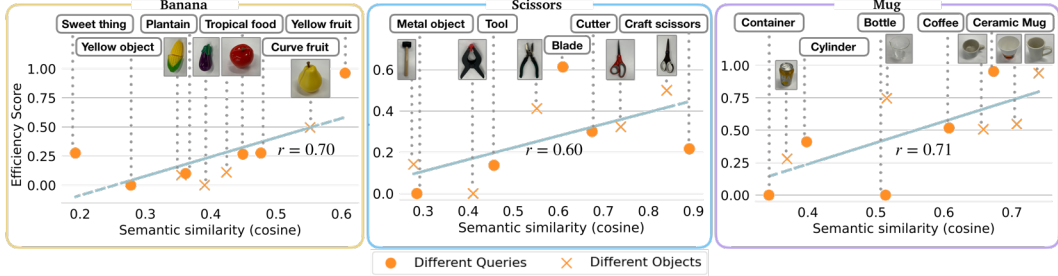
Figure 21: Generalization plots for unseen queries and objects in the same category: (left) banana , (center) scissors , (right) mug . We see a positive correlation in semantic similarity (cosine distance) of the objects/queries with the most similar object present in our training objects, and the efficiency score suggesting the model’s performance.
