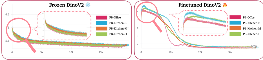
Figure 12: Frozen vs. Finetuned DINOv2 Encoder. Finetuning the DINOv2 encoder generally leads to training instability, negatively impacting performance.
