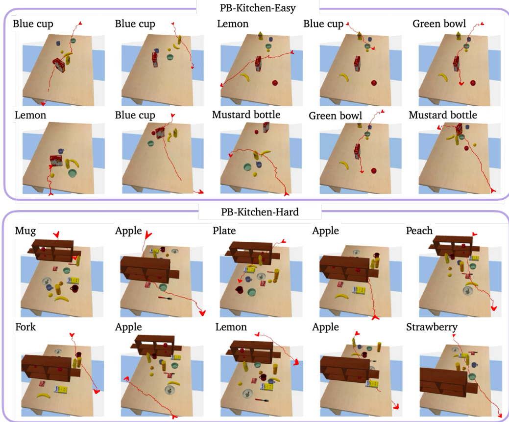
Figure 17: Diffusion policy trajectory visualizations. Top two rows: PB-Kitchen-Easy with easy initial conditions, Bottom two rows: PB-Kitchen-Hard with hard initial conditions. The DP generally moved forward in the direction the robot was initialized at, without showing any intelligent exploration behavior, e.g., looking behind objects.
