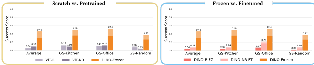
Figure 11: World Model Architecture Ablations in the Gaussian Splatting Scenes. We ablate training the observation encoder from scratch, finetuning, and training the observation encoder with image reconstruction, where ViT-R denotes a ViT trained from scratch with image reconstruction, ViT-NR denote a ViT trained from scratch without image reconstruction, respectively, DINO-Frozen denotes a frozen DINOv2 encoder, DINO-R-FT denotes a finetuned DINOv2 model trained with image reconstruction, and DINO-NR-FT denotes a finetuned DINOv2 encoder trained without image reconstruction. WoMAP uses DINO-Frozen.
