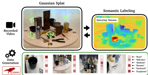
Figure 3: Data Generation. We train Gaussian Splats for each scene and obtain ground truth object locations through semantic labeling [25] for informative view sampling. Each observation is labeled with GroundingDINO [26] to get confidence scores for all training targets.
