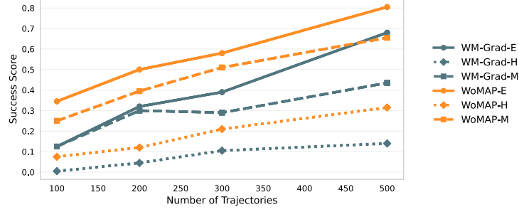
Figure 18: Average success score for different number of trajectories sampled from 50 scenes in the PB-Kitchen-Easy task. We observe a positive correlation between the number of training trajectories and the success rate of WM-Grad and WoMAP across different initial conditions: Easy (E), Medium (M), and Hard (H). With only 200 training trajectories, WoMAP outperforms the VLM and DP baselines (see Figure 6).
