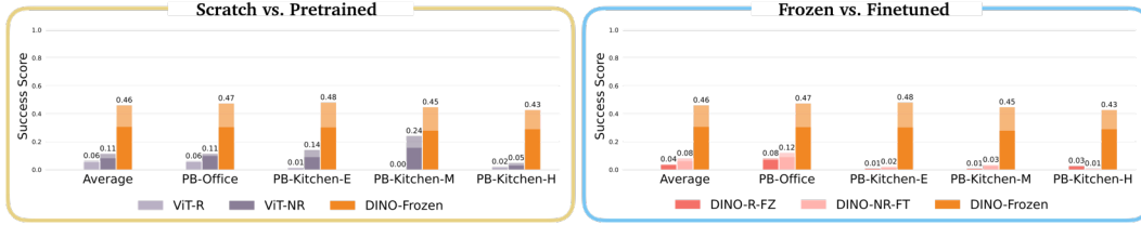
Figure 10: World Model Architecture Ablations in the PyBullet Scenes. We explore training the observation encoder from scratch, finetuning, and training the observation encoder with image reconstruction, where ViT-R denotes a ViT trained from scratch with image reconstruction, ViT-NR denote a ViT trained from scratch without image reconstruction, respectively, DINO-Frozen denotes a frozen DINOv2 encoder, DINO-R-FT denotes a finetuned DINOv2 model trained with image reconstruction, and DINO-NR-FT denotes a finetuned DINOv2 encoder trained without image reconstruction. WoMAP uses DINO-Frozen.
