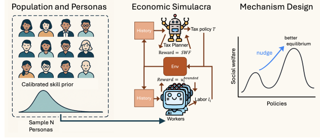
Figure 1: LLM Economist Framework. Left: Population of persona-conditioned agents. Center: Two-level economic simulacra. Right: Mechanism design via successive planner nudges.
